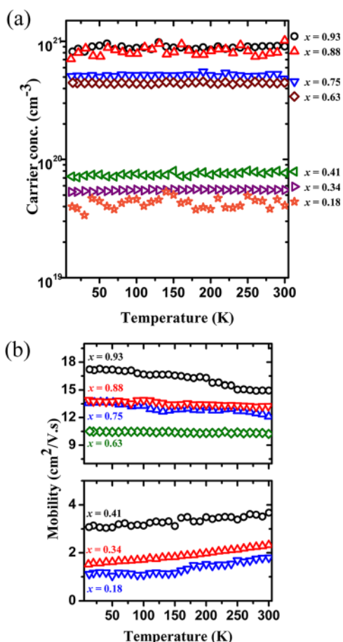
FIG. 2. (Color online) Temperature dependent (a) carrier concentration and (b) mobility values of IGN films with different indium concentrations.
