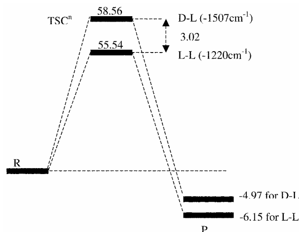
Figure 6. Comparison of the transition state energy level diagram of L-L and D-L phenylalanine peptide bond formation reaction at HF/6-31G level of theory. The relative energies are expressed in kcal/mol. The corresponding imaginary frequencies are noted as well as relative energies of transition states and products relative to the reactants.
