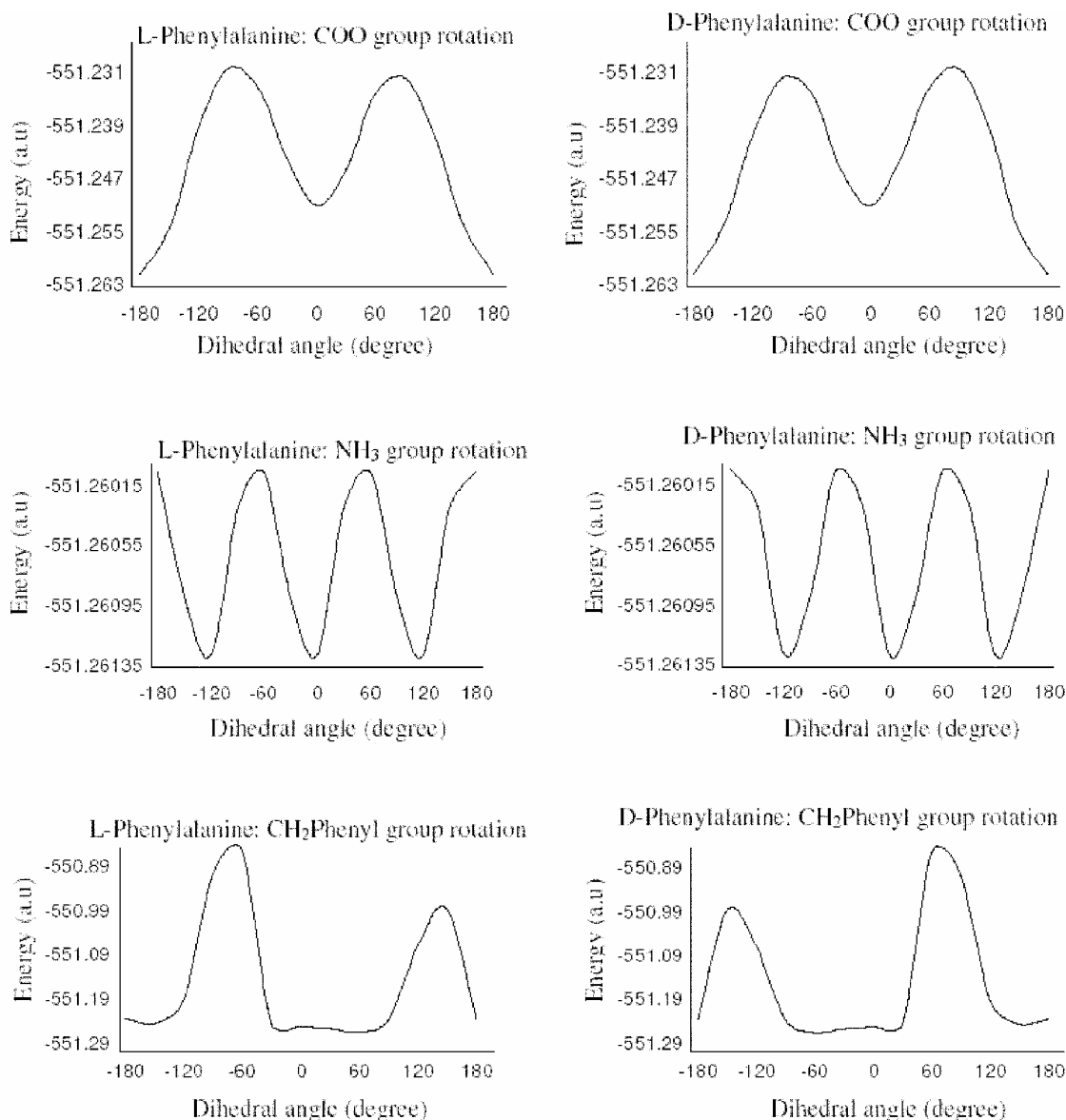
Figure 3. Variation in conformational energy as a function of rotation of COO - , NH 3 + and CH 2 Ph groups for zwitterionic phenyl alanine. The related dihedral angles are O (of COO - )-C (of COO - )-C* (chiral carbon)-N(amine) for the rotation of COO - , H (of NH 3 + )-N (of NH 3 + )-C* (chiral carbon)-C (of CH 2 of CH 2 Ph) for the rotation of NH 3 + , N (of NH 3 + )-C* (chiral carbon)-C (of CH 2 of CH 2 Ph)-C (C of Ph attached to CH 2 ) for the rotation of CH 2 Ph.
