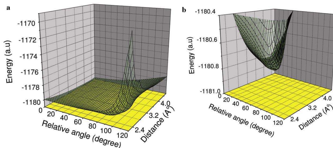
Figure 5. (a) Variation of intermolecular energy as a function of intermolecular distance and orientation of D-L pair of A- and P-terminals in crystal structure of the ribosomal part of the H. marismortui . (PDB ID: 1Q86). The carbon atom attached to t-RNA part is replaced by a methyl group, (b) same plot with enlarged view of the minima region.
