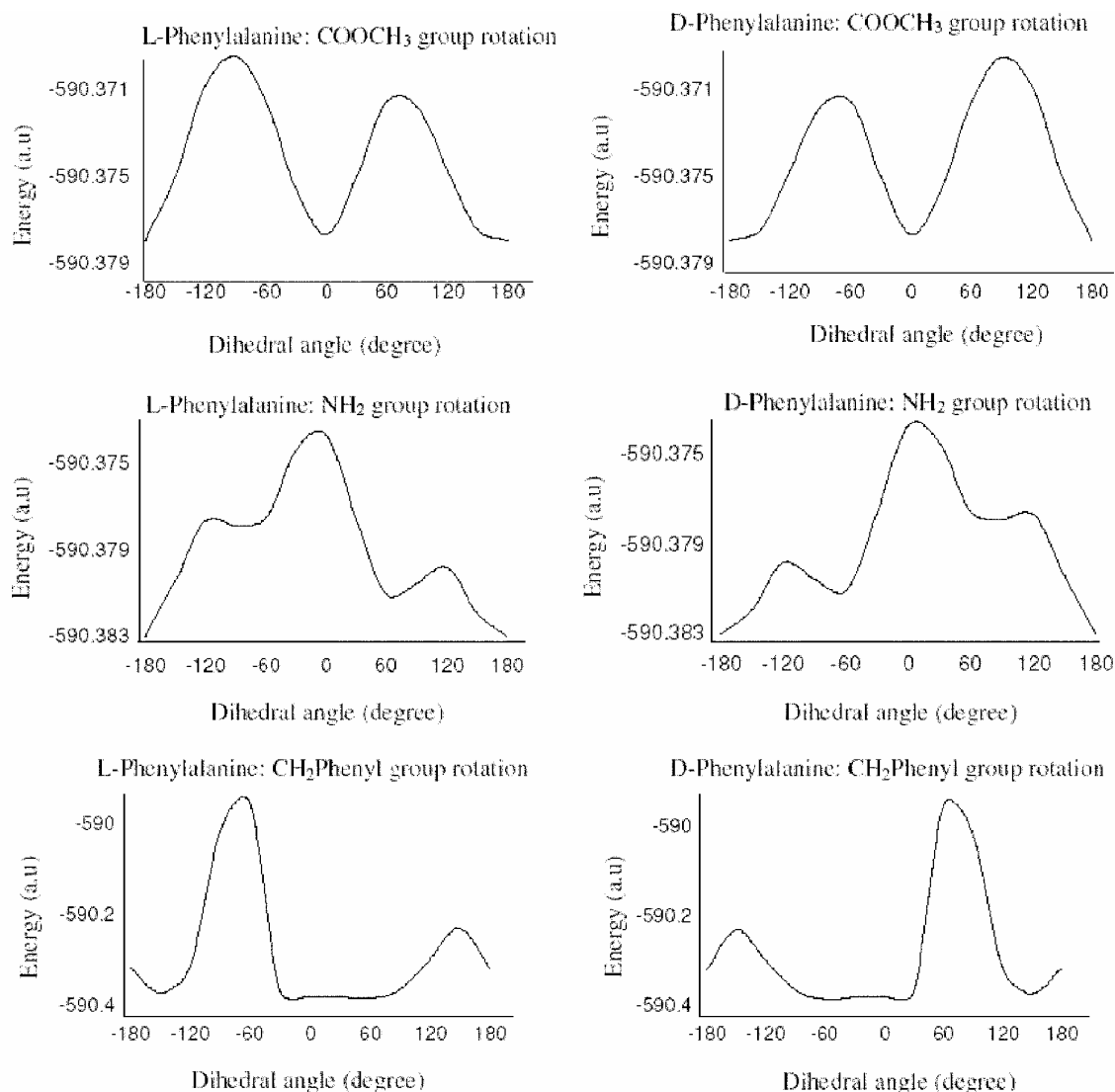
Figure 2. Variation in conformational energy as a function of rotation of COOCH 3 , NH 2 and CH 2 Ph groups for neutral methoxy phenyl alanine. The related dihedral angles are O (of COO)–C (of COO)–C* (chiral carbon)–N(amine) for the rotation of COOCH 3 , H(of NH 2 )–N (of NH 2 )–C* (chiral carbon)–C (of CH 2 of CH 2 Ph) for the rotation of NH 2 , N (of NH 2 )–C* (chiral carbon)–C(of CH 2 of CH 2 Ph)–C (C of Ph attached to CH 2 ) for the rotation of CH 2 Ph.
