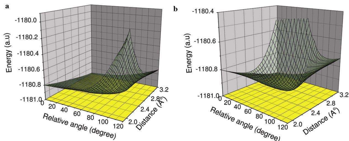
Figure 4. (a) Variation of intermolecular energy as a function of intermolecular distance and orientation of L-L pair of A- and P-terminals in crystal structure of the ribosomal part of the H. marismortui . (PDB ID: 1Q86). The carbon atom attached to t-RNA part is replaced by a methyl group, (b) same plot with enlarged view of the minima region.
