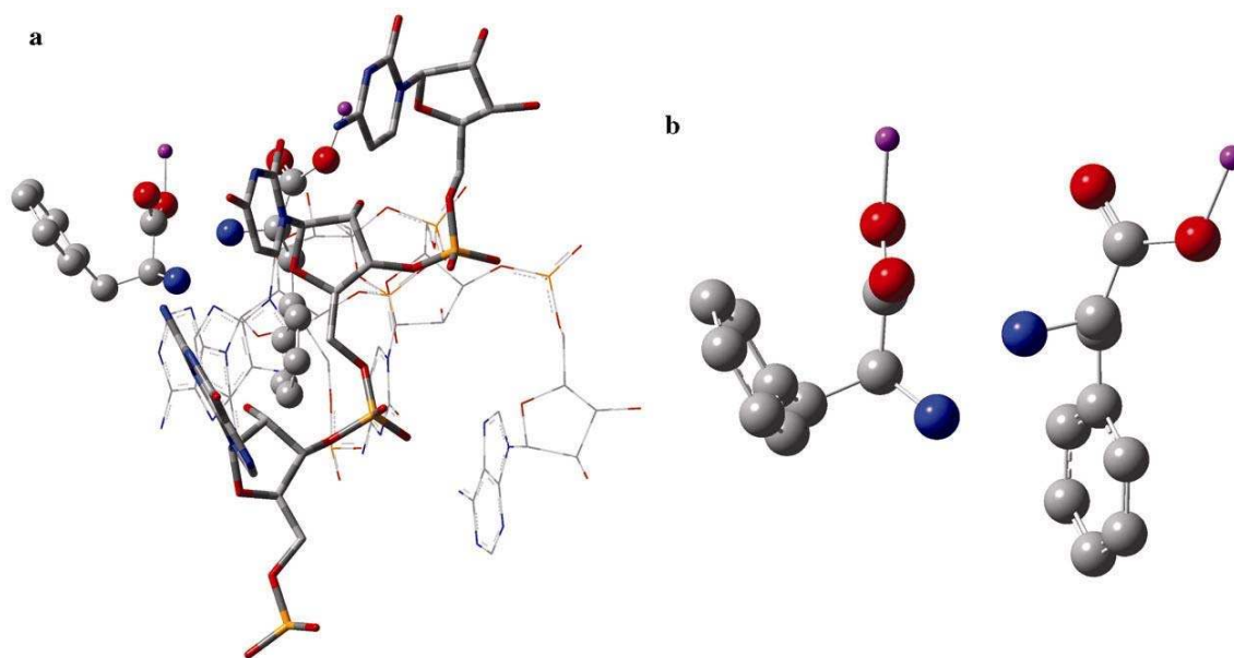
Figure 1. (a) An image of the peptidyl transferase cavity from the crystal structure of CCA-Phe-cap-biotin bound simultaneously at half occupancy to both the A-site and P-site of the 50S ribosomal sub-unit taken from the crystal structure of the ribosomal part of the Haloarcula marismortui (PDB ID: 1Q86). 8 Residues include (all numberings corresponds to scheme as in H. marismortui ): A76 of CCA attached to phenyl alanine at A-terminal, A76 of CCA attached to phenyl alanine at P-terminal, A2485, A2486, C2487, A2488, U2620, A2637, G2540, U2451 and C2452, (b) enlarged view of A- and P-terminals in crystal structure of the ribosomal part of the H. Marismortui (PDB ID: 1Q86).
