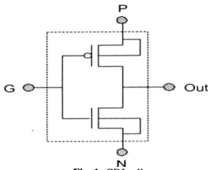
Fig. 1: GDI cell
