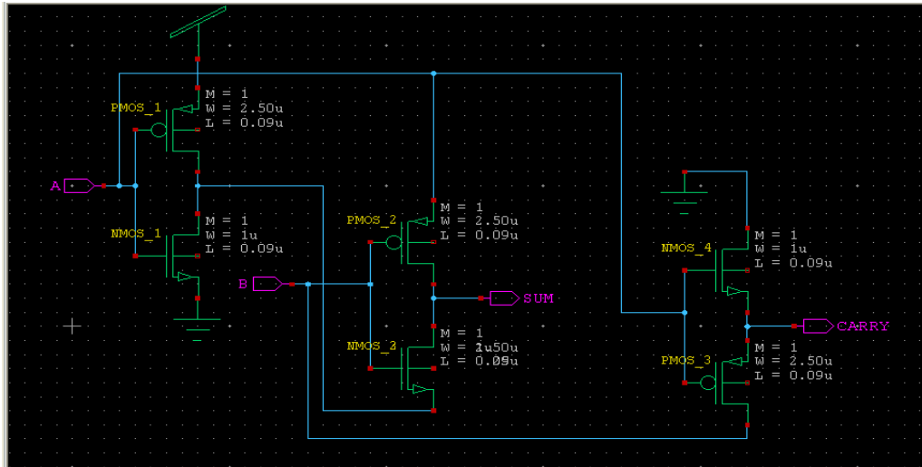
Fig. 5: Half Adder construction in Tanner EDA tool
