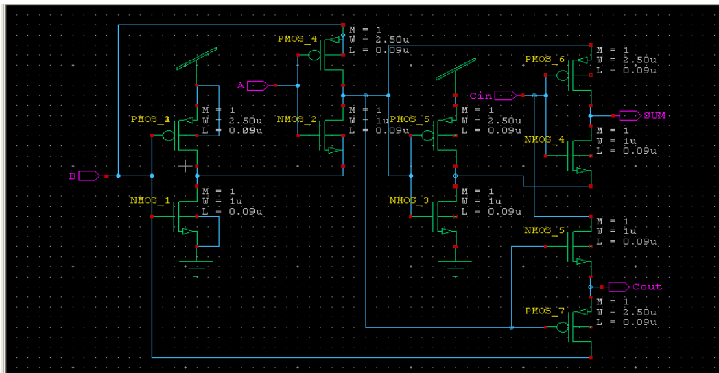
Fig. 6: Full Adder construction in Tanner EDA tool
