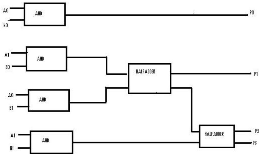
Fig. 3: 2-bit Vedic Multiplier Architecture
