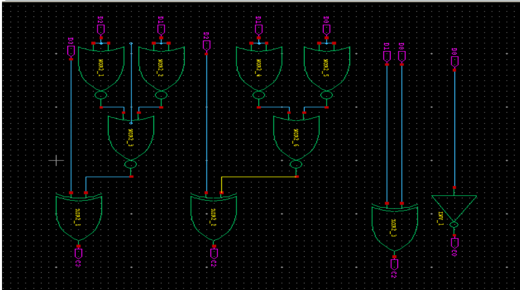
Fig. 7: Carry save Adder Schematic Diagram
