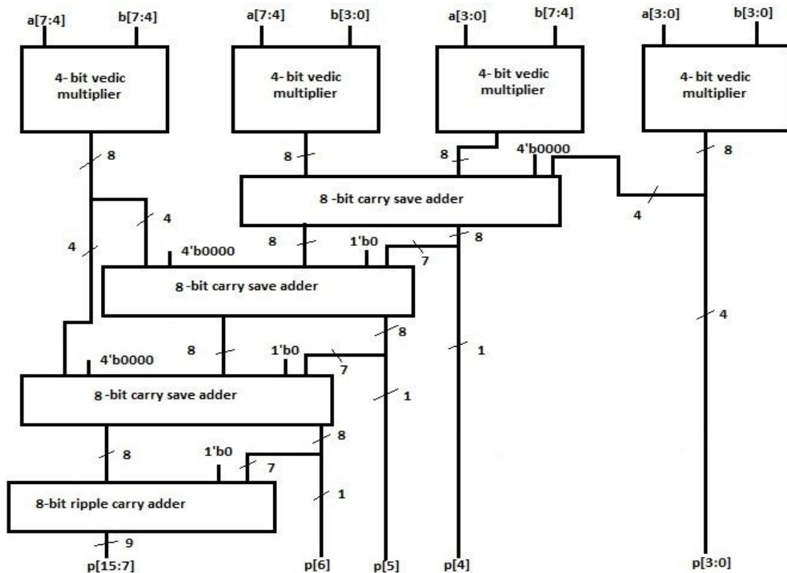
Fig. 4: 8-bit Vedic Multiplier Architecture
