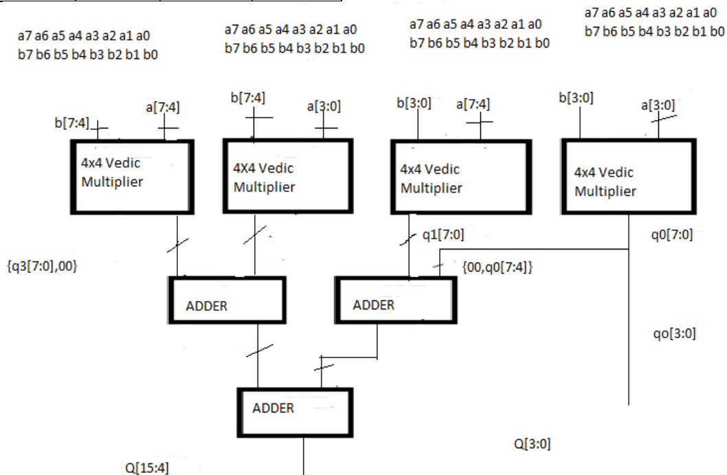
Fig. 2: 4-Bit Vedic Multiplier Architecture
