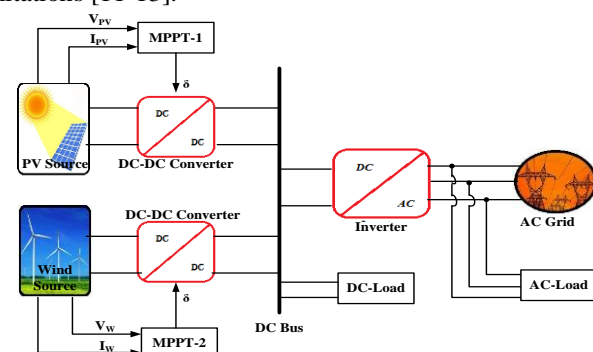
FIGURE 1. Hybrid PV and wind system basic topology
