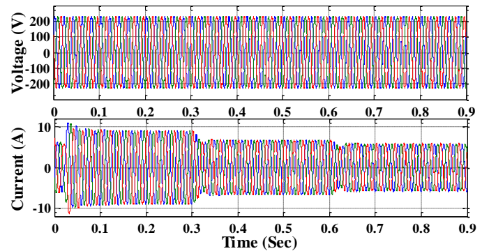
FIGURE 19. Grid voltage, current
