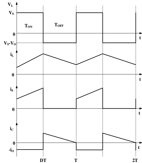
FIGURE 7. Switching waveform of Boost Converter
