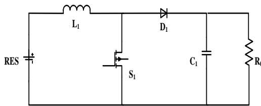
FIGURE 6. Equivalent circuit of conventional Boost converter
