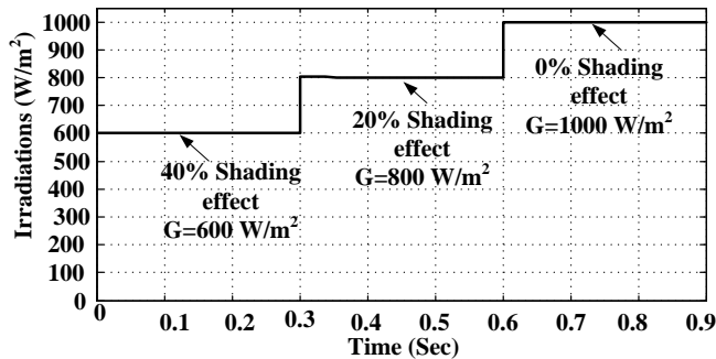
FIGURE 11. Considered solar irradiation pattern for PV system
