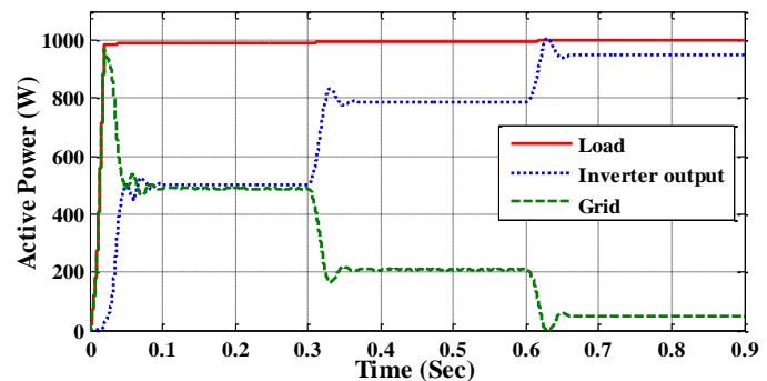
FIGURE 20. Active power
