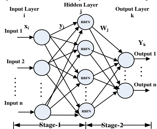
FIGURE 8. Architecture of RBFN
