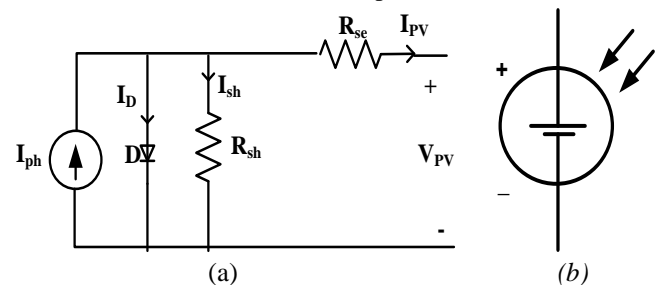
FIGURE 3. PV cell single diode model (a) equivalent circuit, (b) Symbolic representation
