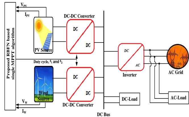
FIGURE 2. Proposed single MPPT topology for hybrid PV and wind system
