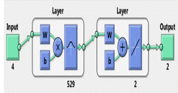
FIGURE 9. RBFN based single MPPT architecture for hybrid system
