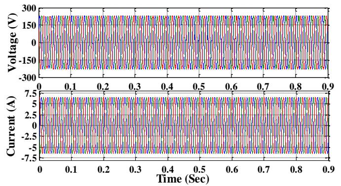
FIGURE 18. Load voltage, current
