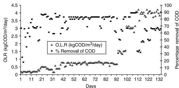
Figure 4 | Performance of UAFFR with varying organic loading rate (OLR).
