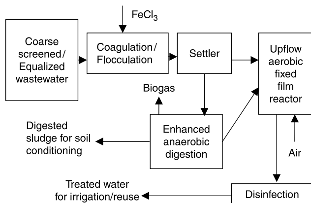
Figure 1 | Process flow diagram of ecologically sustainable wastewater treatment system.
