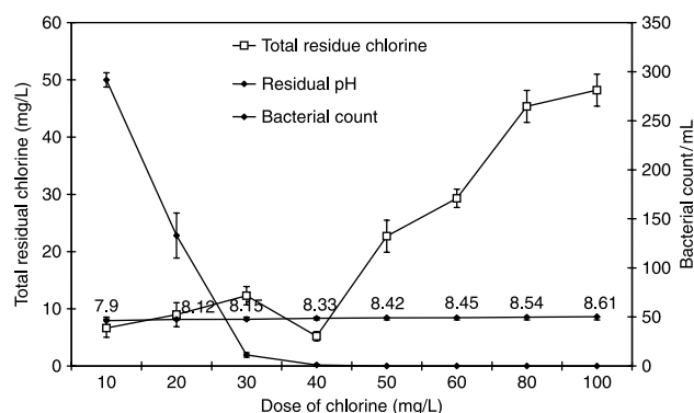
Figure 5 | Break point chlorination of UAFFR effluent.
