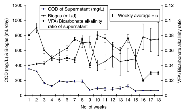
Figure 3 | Performance of anaerobic digester.
