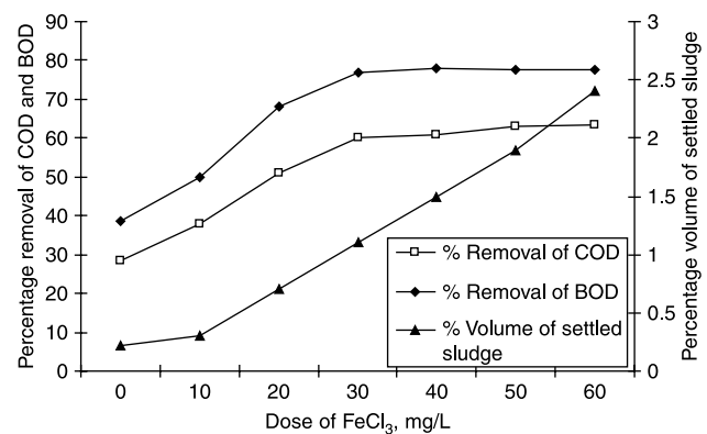
Figure 2 | Results of enhanced primary treatment.
