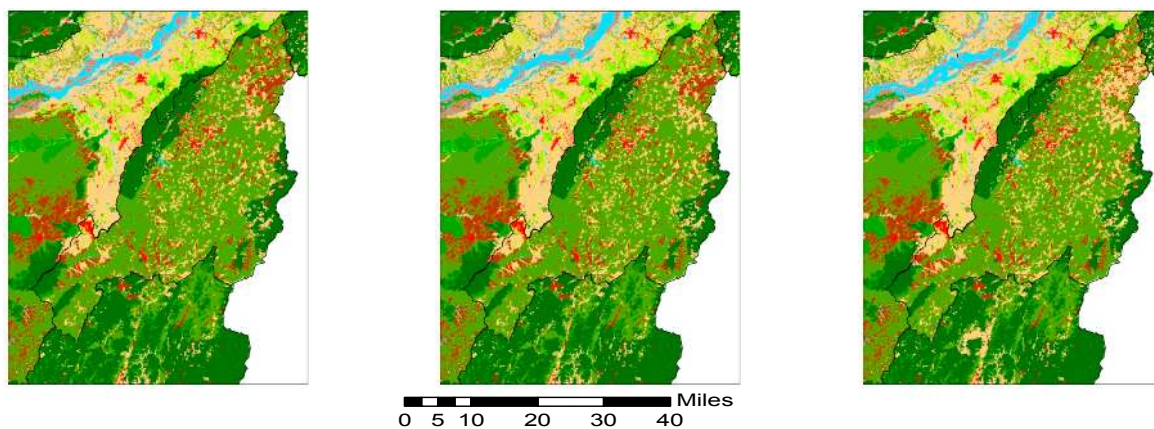
B. Decrease in area under evergreen forests and increase in cropland areas in Manipur
