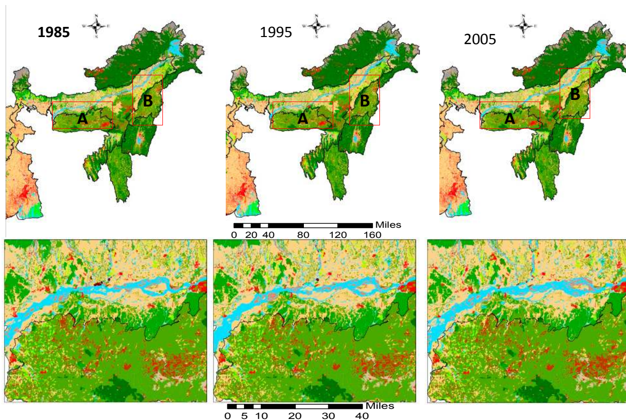
A. Decrease in forest cover types in Assam valley and Garo hills due to felling and shifting cultivation
