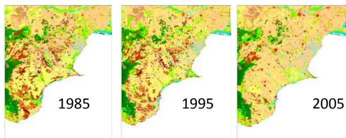
C. Decrease in forest cover and Wasteland and increase in cropland in the Cauvery river basin
