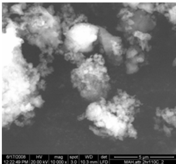
Figure 10. Scanning electron microscope image revealing similar morphology of the powders heat treated at different temperatures.
