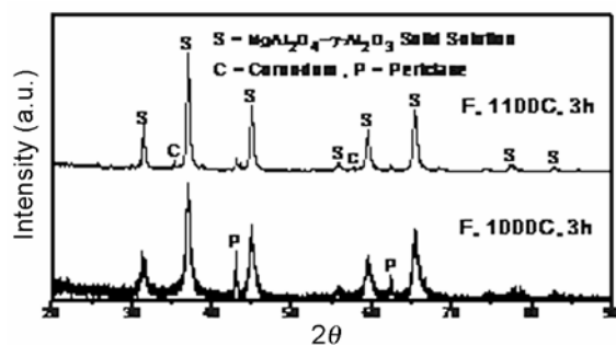
Figure 4. XRD spectra of powder F calcined at 1000°C (3 h) and 1100°C (3 h).
