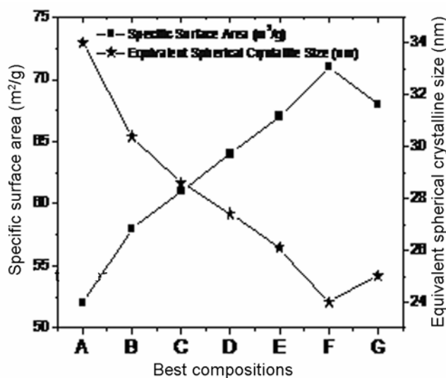
Figure 7. BET specific surface area and equivalent spherical crystallite size of 1000°C (3 h) heat treated powders.
