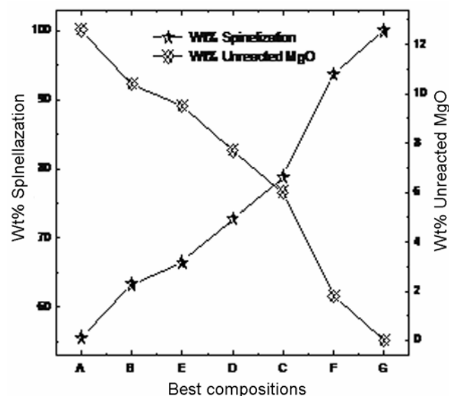
Figure 8. Graph revealing unconverted MgO as index for MgAl 2 O 4 formation in the processed powders calcined at 1100°C (3 h).
