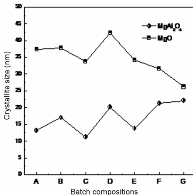
Figure 6. Calculated crystallite size (by Scherrer equation) of processed powders calcined at 1000°C (3 h) from XRD peaks of MgAl 2 O 4 and MgO.
