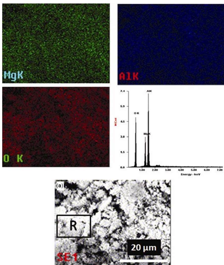
Figure 11. Distribution of elements magnesium, aluminium and oxygen in 1000°C (3 h) heat treated powder G i.e. image (a). The EDS is of region R.
