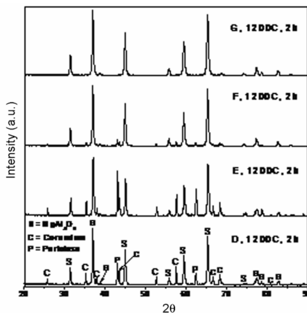
Figure 9. X-ray diffraction spectral patterns of powders D, E, F and G heat treated at 1200°C (2 h).
