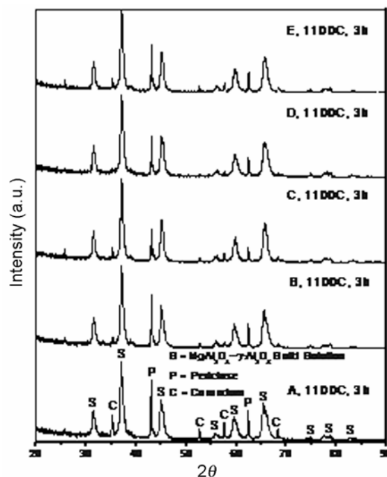
Figure 3. XRD spectra at 1100^\circ C (3 h) of powders A, B, C, D and E. Compared to 1000^\circ C (3 h) XRD spectra, exsolution of corundum from spinel solid solution has occurred to a certain extent.
