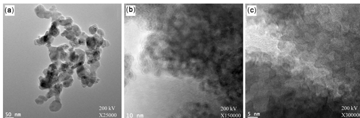
Figure 12. TEM of powder G (a) Size of the agglomerate at 1000°C (3h) under lower magnification; (b) Nano size crystallites when part of the 1000°C (3 h) calcined agglomerate, i.e. image (a), is viewed at higher magnification; (c) Nano size crystallites of spinel at 1100°C (3 h).
