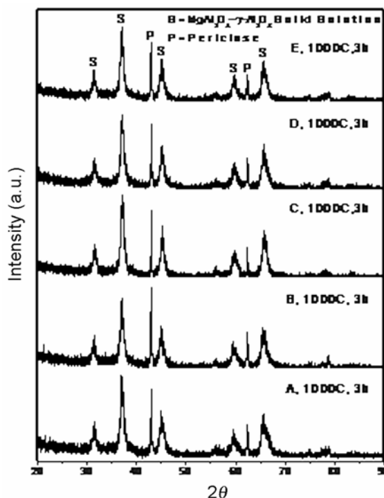
Figure 2. XRD spectra at 1000^\circ C (3 h) of powders A, B, C, D and E. Unconverted alumina ( \gamma-Al_2O_3 ) exists as solid solution with MgAl_2O_4 .
