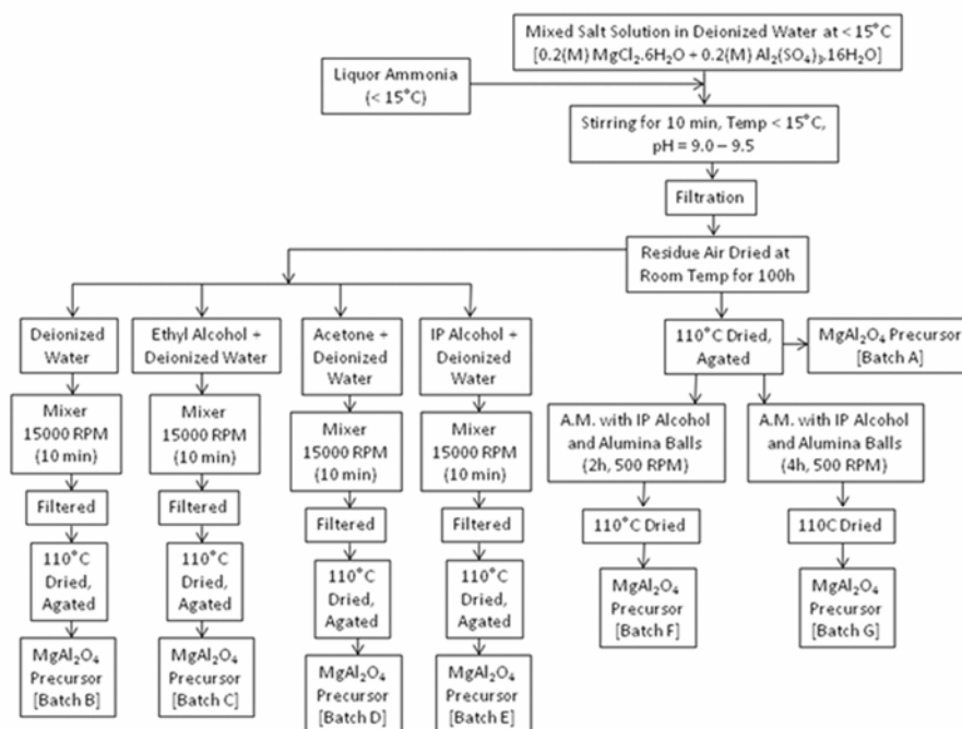
Figure 1. Flow chart depicting the preparation procedure of processed spinel precursors through coprecipitation technique.
