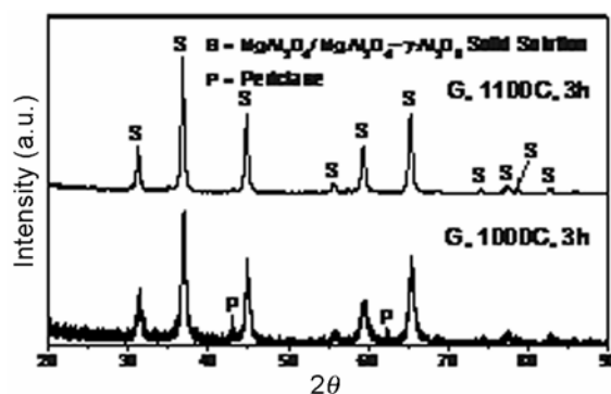
Figure 5. XRD spectra of powder G calcined at 1000°C (3 h) and 1100°C (3 h).
