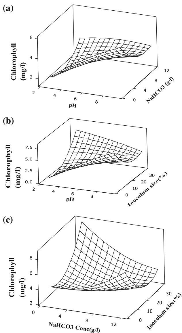
Fig. 4 Surface plot for chlorophyll (mg/l). a Conc. of NaHCO 3 (g/l), pH. b Inoculum size (%), pH. c Inoculum size (%), Conc. of NaHCO 3 (g/l)
