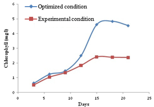
Fig. 2 Growth profile of microalgae under optimized condition [pH 8, \text{NaHCO}_3 3.33 (g/l), inoculum size -30 (%)] and experimental condition
