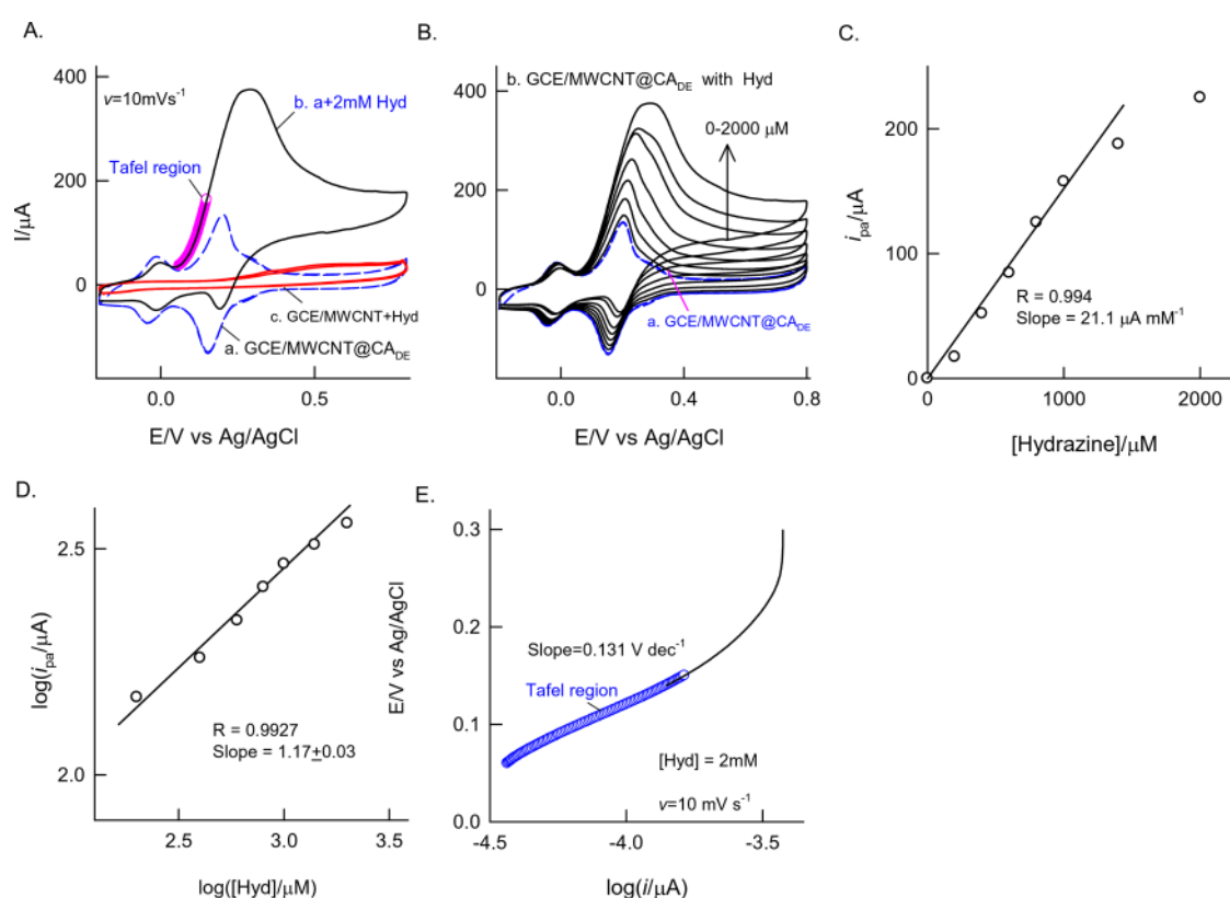
Figure 8. (A) CV responses of GCE/MWCNT@CA DE (a) without and (b) with 2 mM hydrazine at \nu = 10 \text{ mV s}^{-1} in pH 7 PBS. The inset plot is a Tafel region. Curve c is a control CV of the GCE/MWCNT with 2 mM hydrazine. (B) Effect of hydrazine concentration on the CV response of GCE/MWCNT@CA DE at \nu = 10 \text{ mV s}^{-1} in pH 7 PBS. Plots of (C) i_{pa} vs Hyd concentration, (D) \log i_{pa} vs \log[\text{Hyd}] , and (E) E vs \log i (Tafel plot).
