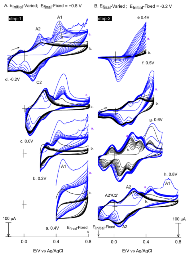
Figure 3. Effect of potential on the continuous CV response of the GCE/MWCNT (freshly prepared electrodes) with 9\text{ mM Ph-2-OCH}_3 in \text{pH } 7\text{ PBS} at \nu = 50\text{ mV s}^{-1} . (A) CV experiments with a fixed final potential of 0.8\text{ V} and varying switching initial potentials of (a) 0.4 , (b) 0.2 , (c) 0 , and (d) -0.2\text{ V} vs Ag/AgCl (step 1). (B) CV experiments with a fixed initial potential of -0.2\text{ V} and varying final potentials of (e) 0.4 , (f) 0.5 , (g) 0.6 , and (h) 0.8\text{ V} vs Ag/AgCl (step 2).
