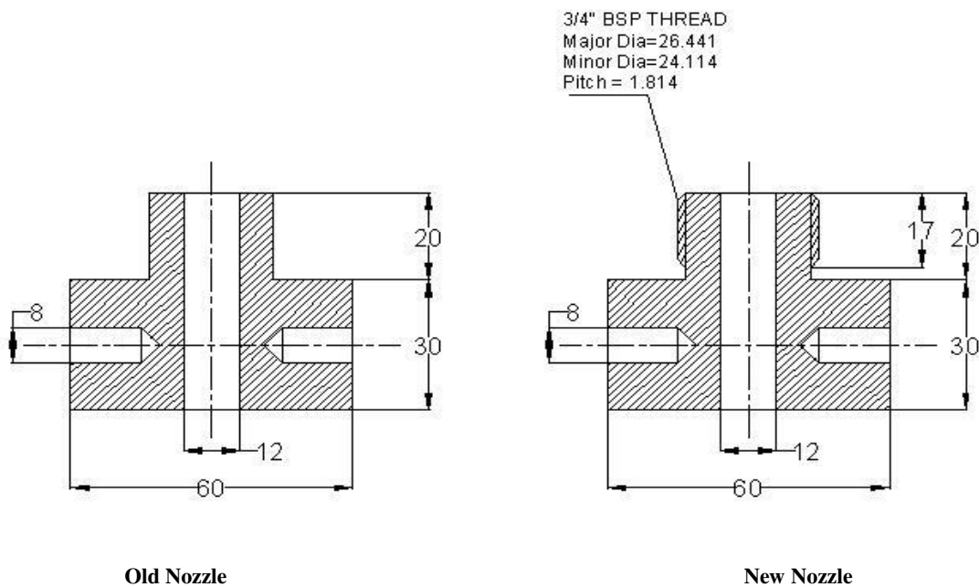
Figure 7. Old Nozzle and Threaded Nozzle
