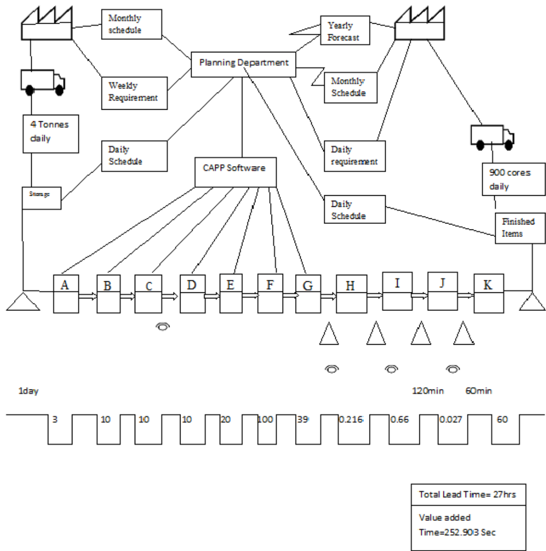
Figure. 10 Future stream map
