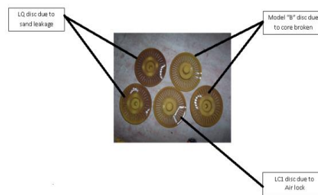
Figure 3. Sample of rejected cores
