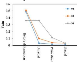
Figure 10. Twin decay of brass in different strain path with different specimen thickness.
