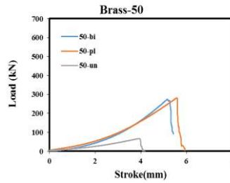
Figure 5. Punch stroke versus load plot for 50 \mu\text{m} thickness brass material.
