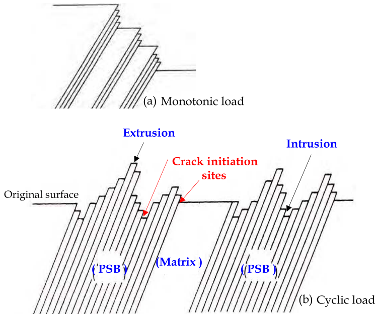
Fig. 9. Schematic of slip under (a) monotonic load and (b) cyclic load [21, p. 13]
