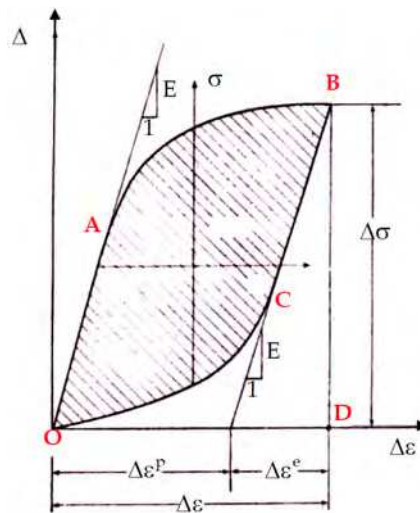
Fig. 8. Hysteresis loop for a masing material
