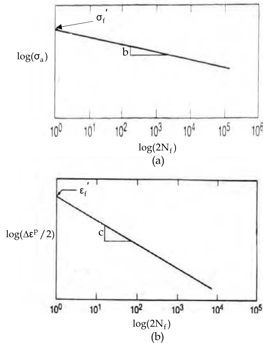
Fig. 4. Stress and strain amplitudes vs number of cycle reversals to failure
