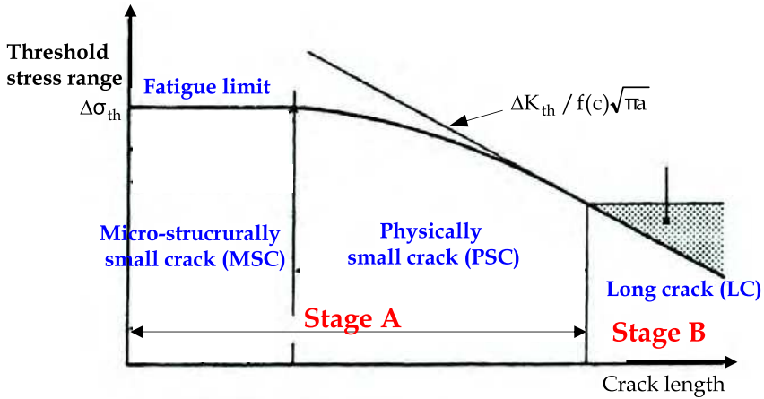
Fig. 11. Three regimes of crack size [21, p. 419]
