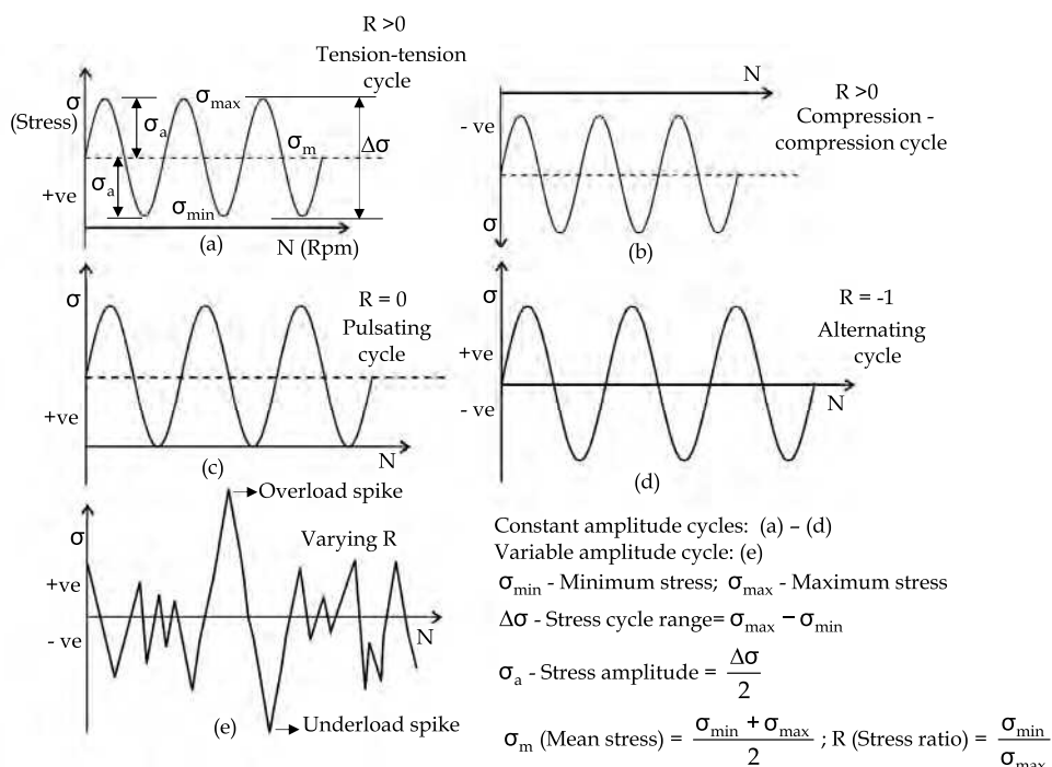
Fig. 2. Types of fatigue cycles
