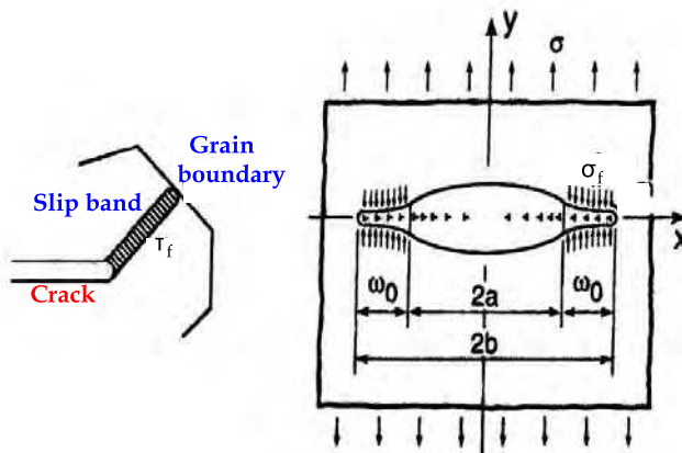
Fig. 15. Schematic of slip band model [21, p. 430]
