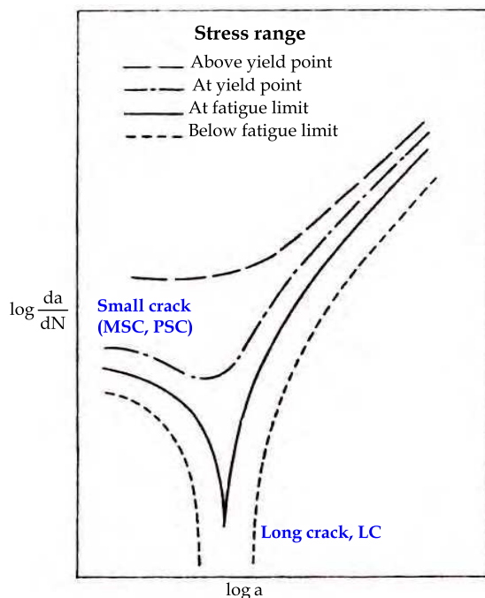
Fig. 13. Crack behavior vs applied cyclic stress [21, p. 416]
