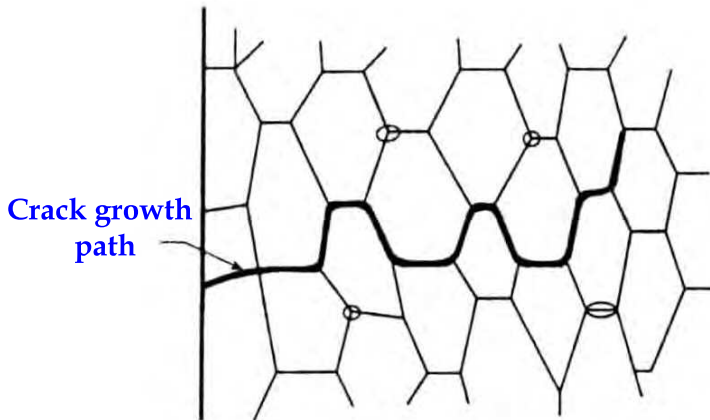
Fig. 20. Crack growth along grain boundaries at high temperature
