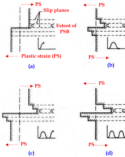
Fig. 14. Stages of small crack growth [21, p. 421]
