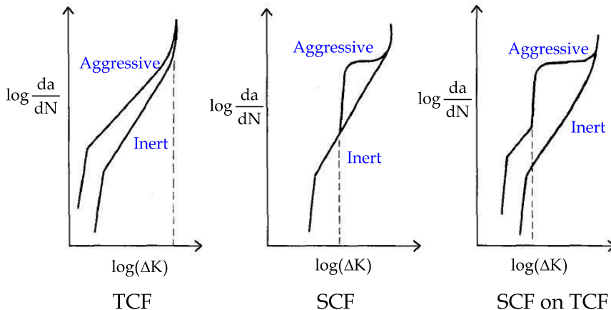
Fig. 19. Types of corrosion fatigue
