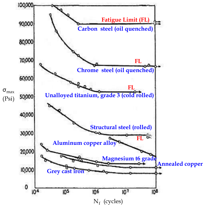
Fig. 3. S-N curves of various metals
