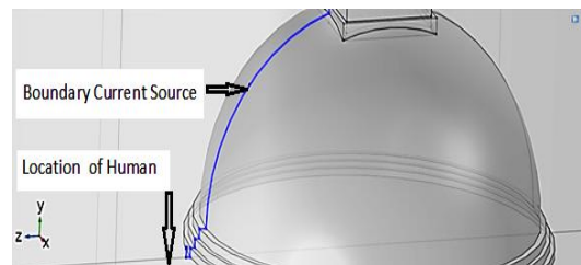
FIGURE 27. Boundary current source and its location in stupas during simulation and analysis
