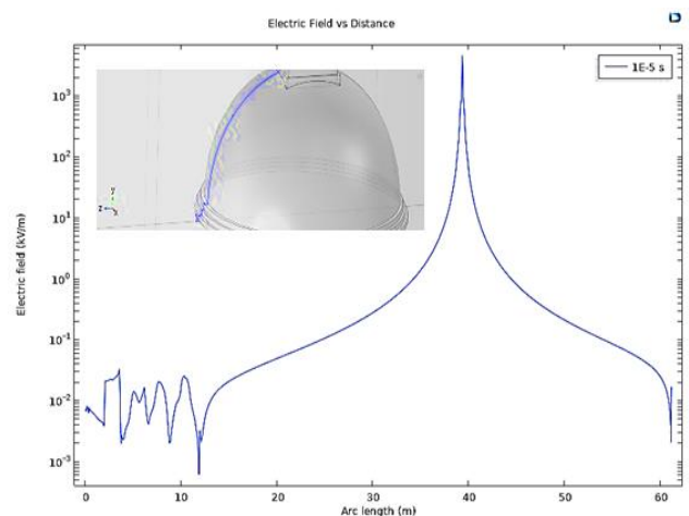
FIGURE 28. Electric field distribution during lightning strike on Ruwanweliseya
