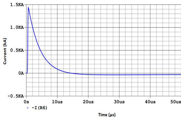
FIGURE 40. Current waveforms of human touch potential due to lightning on monument with earthing resistance of 5 \Omega
