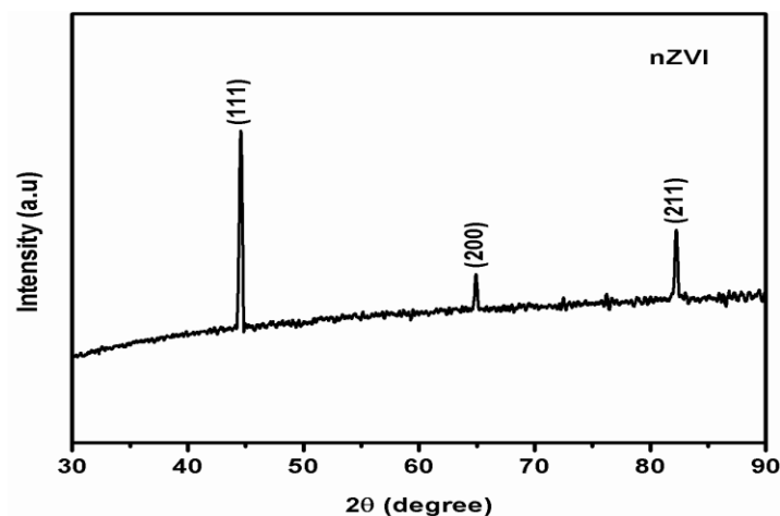
Fig. 1: X-Ray diffraction pattern of n\text{Fe}^0 .
