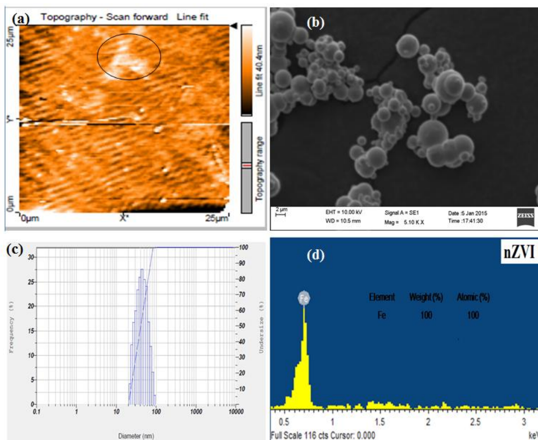
Fig. 2: Characterization studies of n\text{Fe}^0 . (a) AFM image; (b) SEM image; (c) histogram showing particle size distribution and (d) EDAX spectrum.
