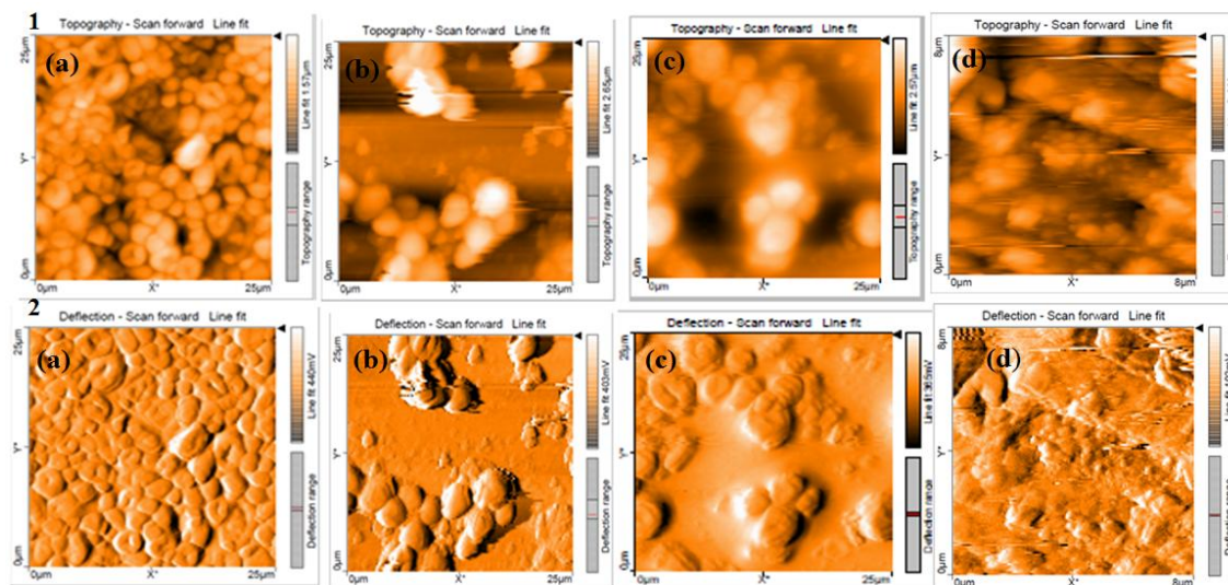
Fig. 4: AFM images of Candida sp. SMN04. (a) Native yeast cells; (b) yeast cells grown with 25mg/mL of n\text{Fe}^0 ; (c) yeast cells grown with 50 mg/mL of n\text{Fe}^0 ; (d) yeast cells grown with 75 mg/mL of n\text{Fe}^0 showing topography (1) and deflection (2) of each image.
