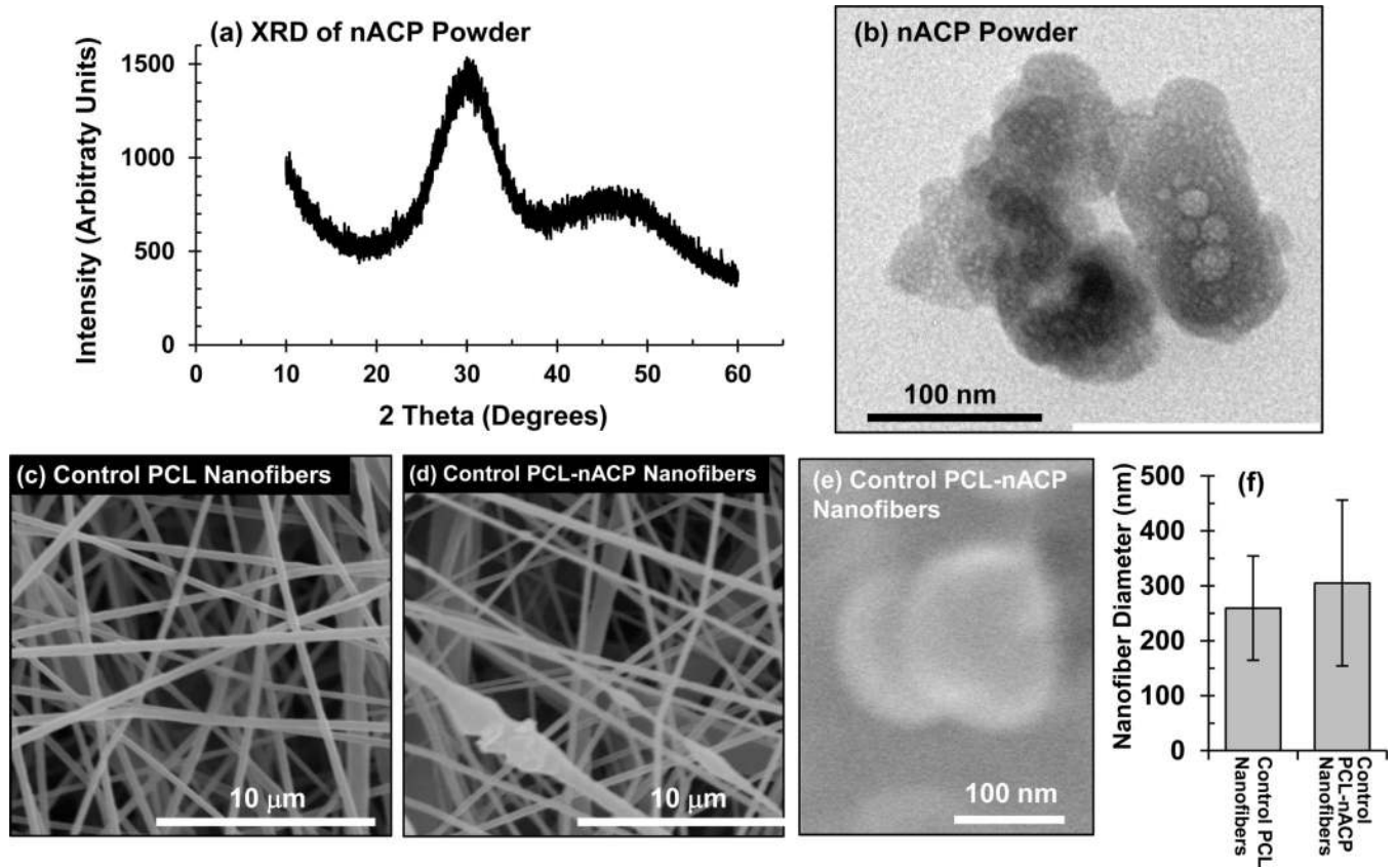
Figure 3. (a) XRD of nACP powder. (b) TEM of nACP particles. (c,d) SEM of control PCL (0 mass percent nACP) and PCL-nACP nanofibers (24 mass percent nACP). (e) Higher magnification SEM showing nACP particle on the surface of a control PCL-nACP nanofiber. (f) The diameter of control PCL and PCL-nACP nanofibers as determined by SEM (error bars are S.D., n = 10 ) are not significantly different [t-test, P > 0.05 ].
