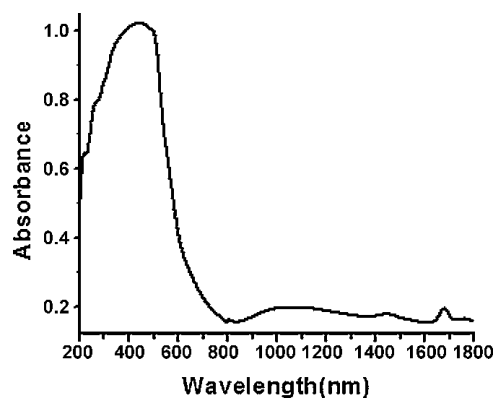
Fig. 6. Diffuse reflectance spectrum of [\text{Ni}^{\text{II}}(\text{L})(\text{Cl})(\text{H}_2\text{O})_2] \cdot \text{H}_2\text{O} .
