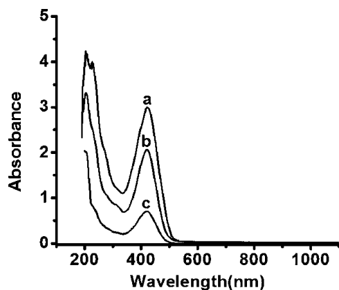
Fig. 4. UV-vis spectra of: (a) the [\text{Ni}^{\text{II}}(\text{L})(\text{Cl})(\text{H}_2\text{O})_2] \cdot \text{H}_2\text{O} , (b) [\text{Ru}^{\text{II}}(\text{L})(\text{Cl})(\text{H}_2\text{O})_2] \cdot \text{H}_2\text{O} , and (c) ligand in acetonitrile.
