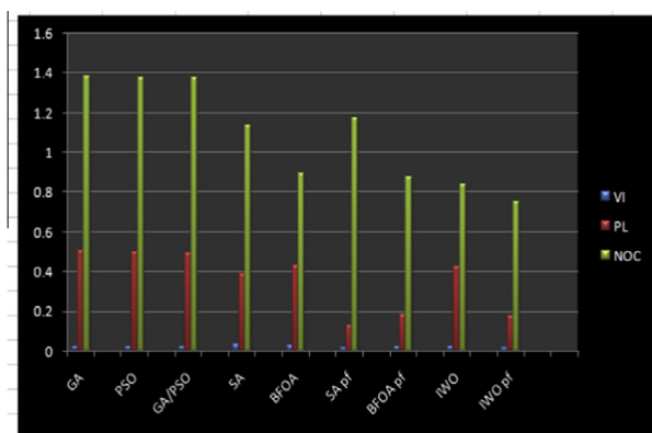
Figure 1 Comparison of performances of IWO for IEEE-33 bus system with other methods [20].
