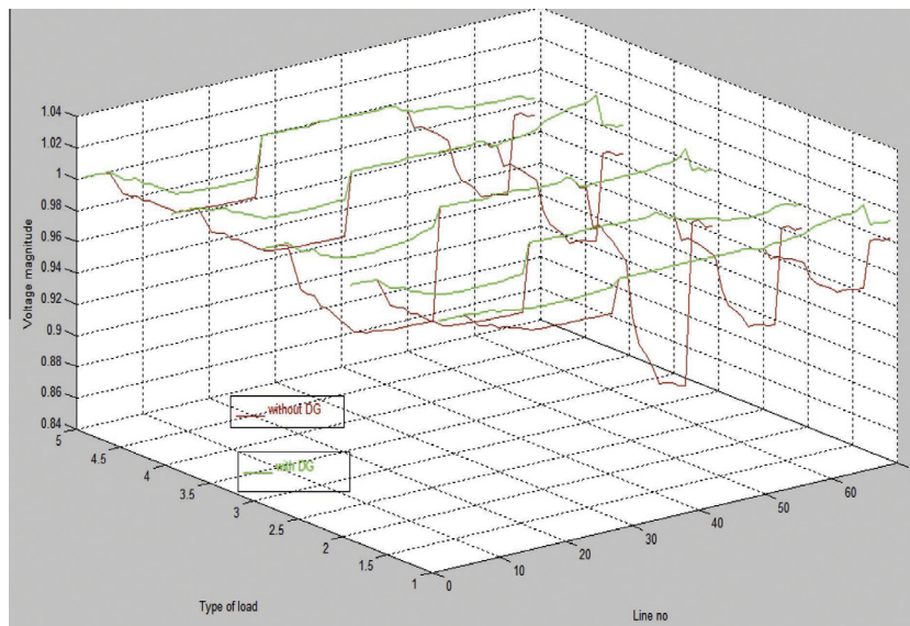
Figure 5 Comparison of voltage magnitude with and without DGs.
