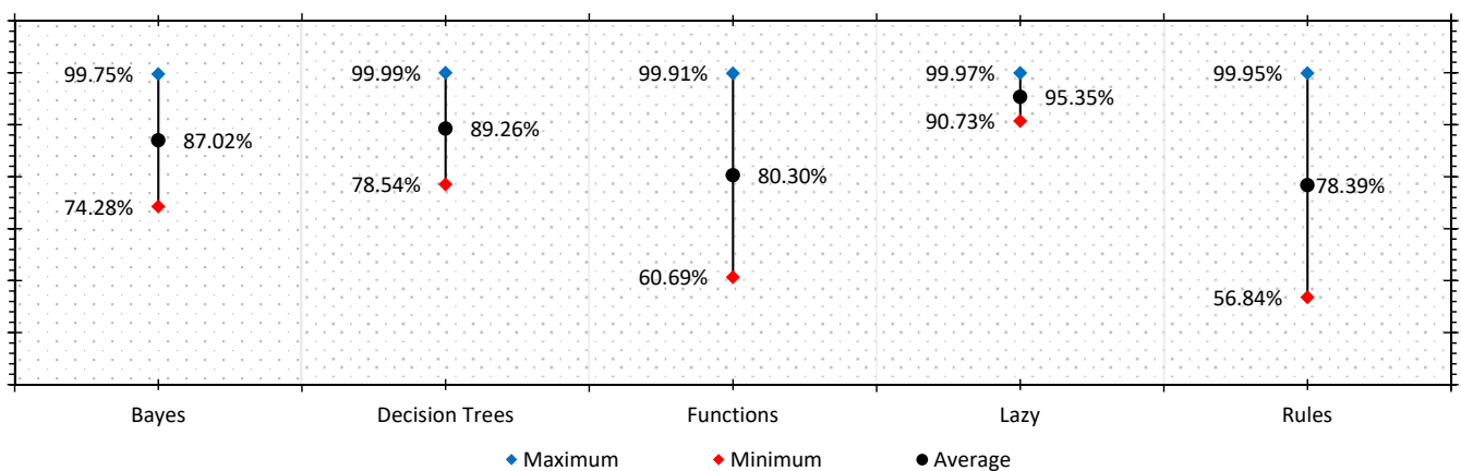
Figure 2. Comparison of classification accuracy in various classifier groups found in the literature.
