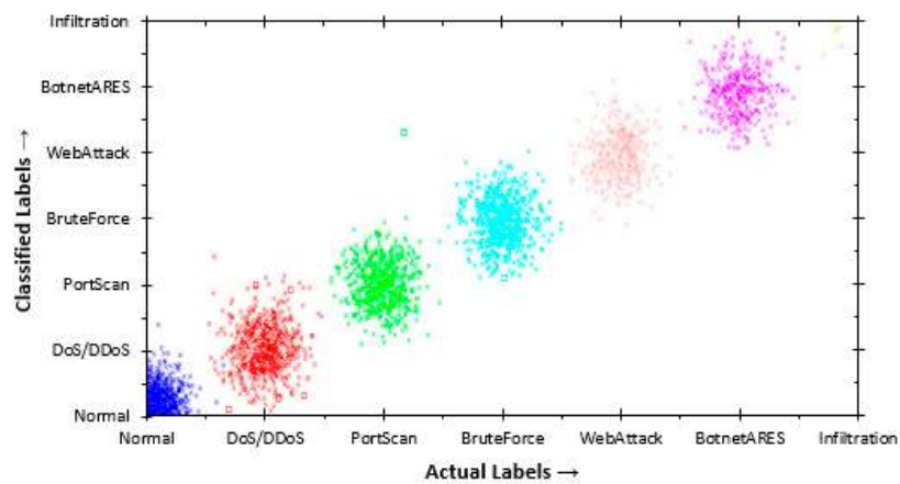
Figure 14. Classification of J48Consolidated on CICIDS2017 dataset.
