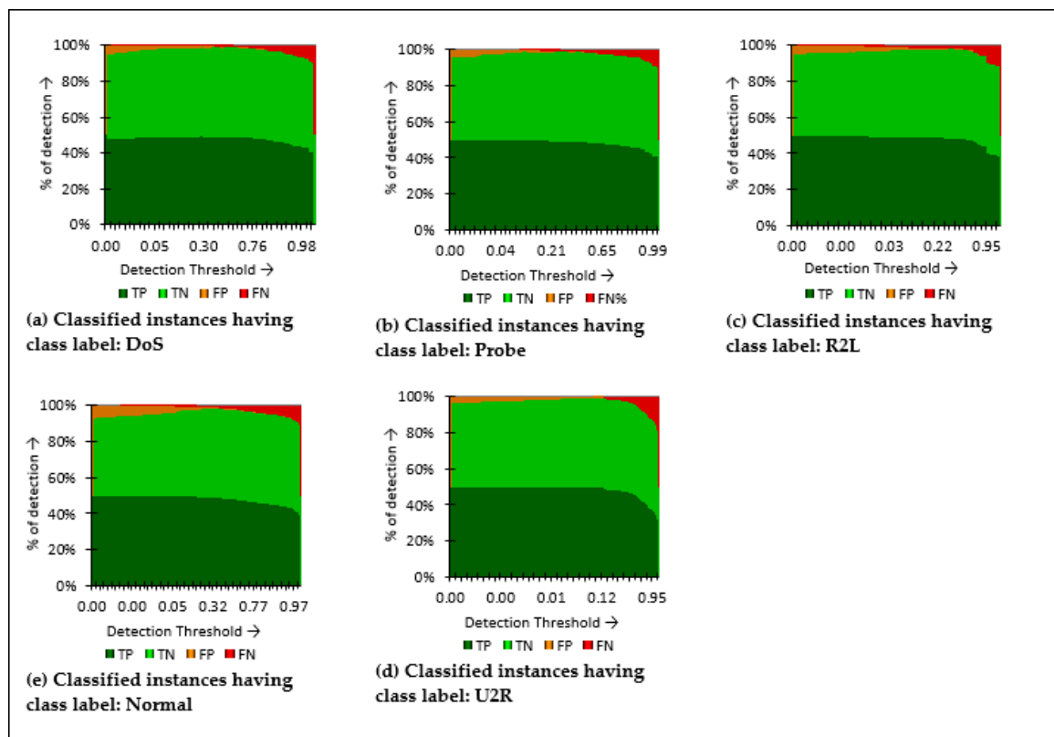
Figure 9. Detection (%) of attacks and normal class labels of NSL-KDD multi-class dataset.
