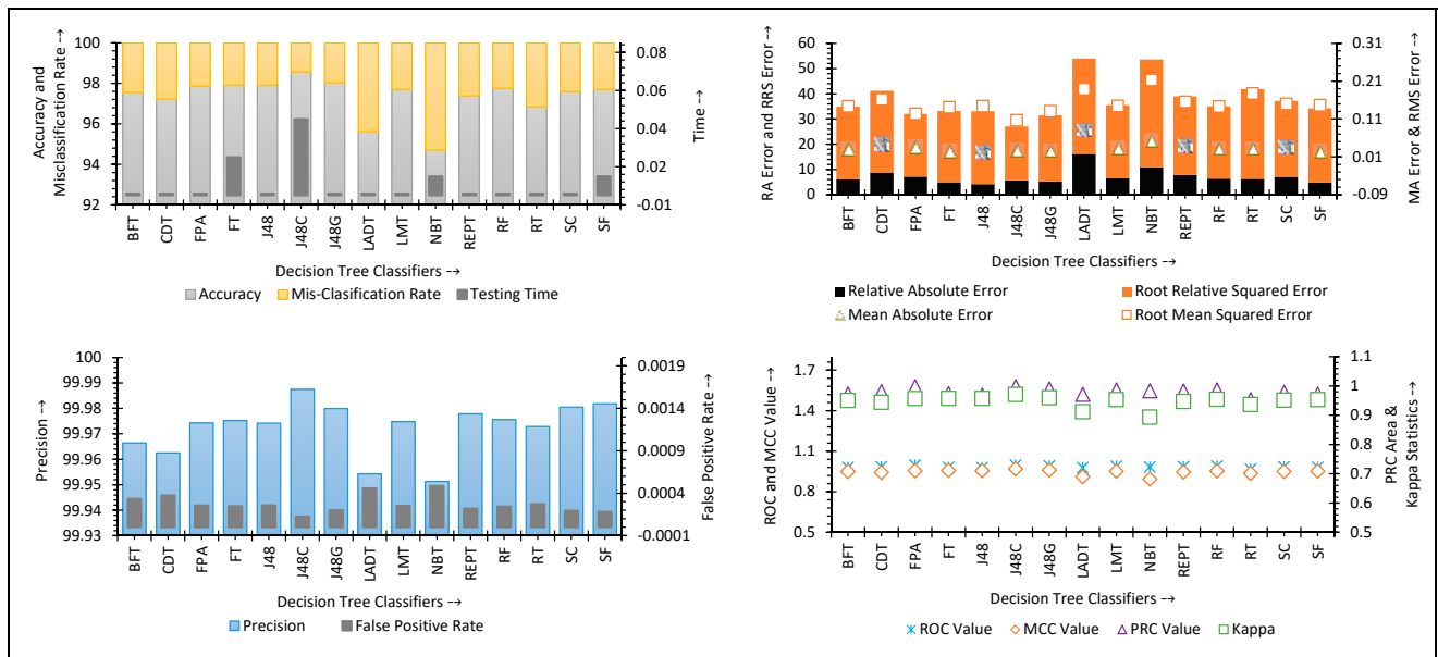
Figure 6. Performance of decision tree classifiers for ISCXIDS2012 dataset.
