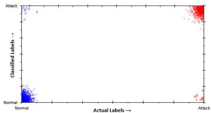
Figure 13. Classification of J48Consolidated on ISCXIDS2012 dataset.
