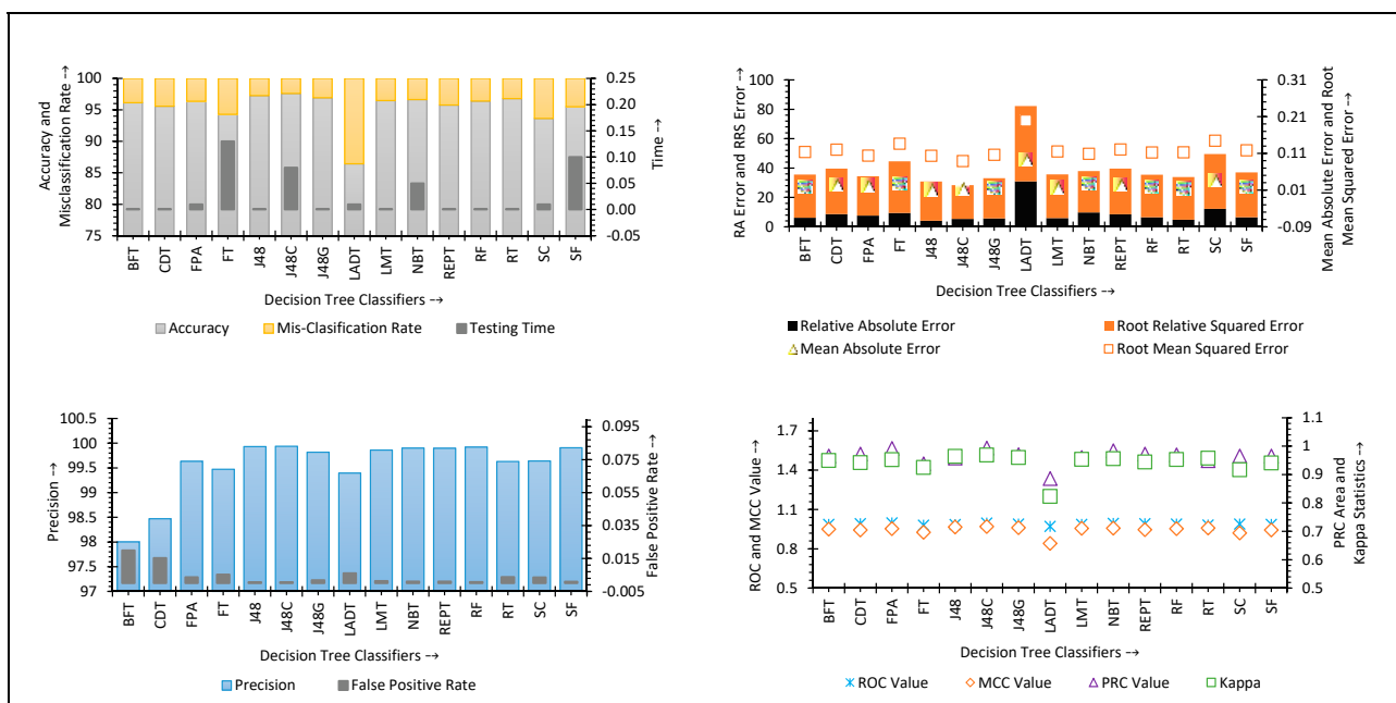
Figure 5. Performance of decision tree classifiers for NSLKDD dataset.
