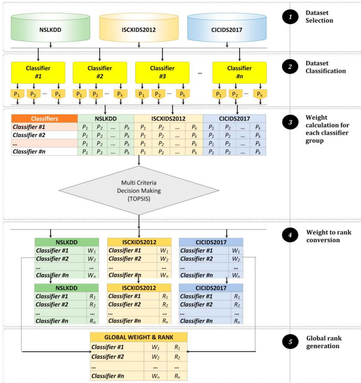
Figure 3. The methodology of classification to rank allocations of supervised classifiers.
