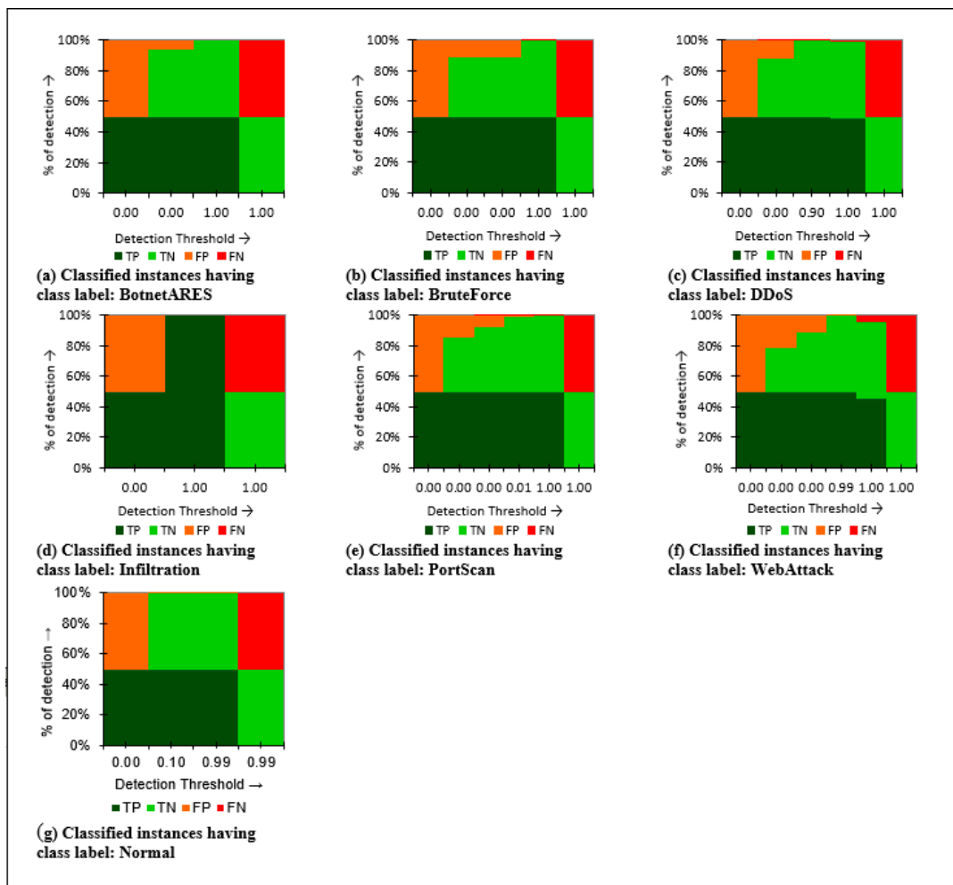
Figure 11. Detection (%) of attacks and normal class labels of CICIDS2017 multi class dataset.
