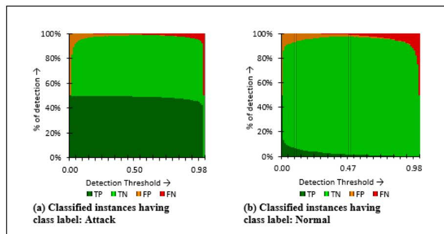
Figure 10. Detection (%) of attacks and normal class labels of ISCXIDS2012 binary class dataset.
