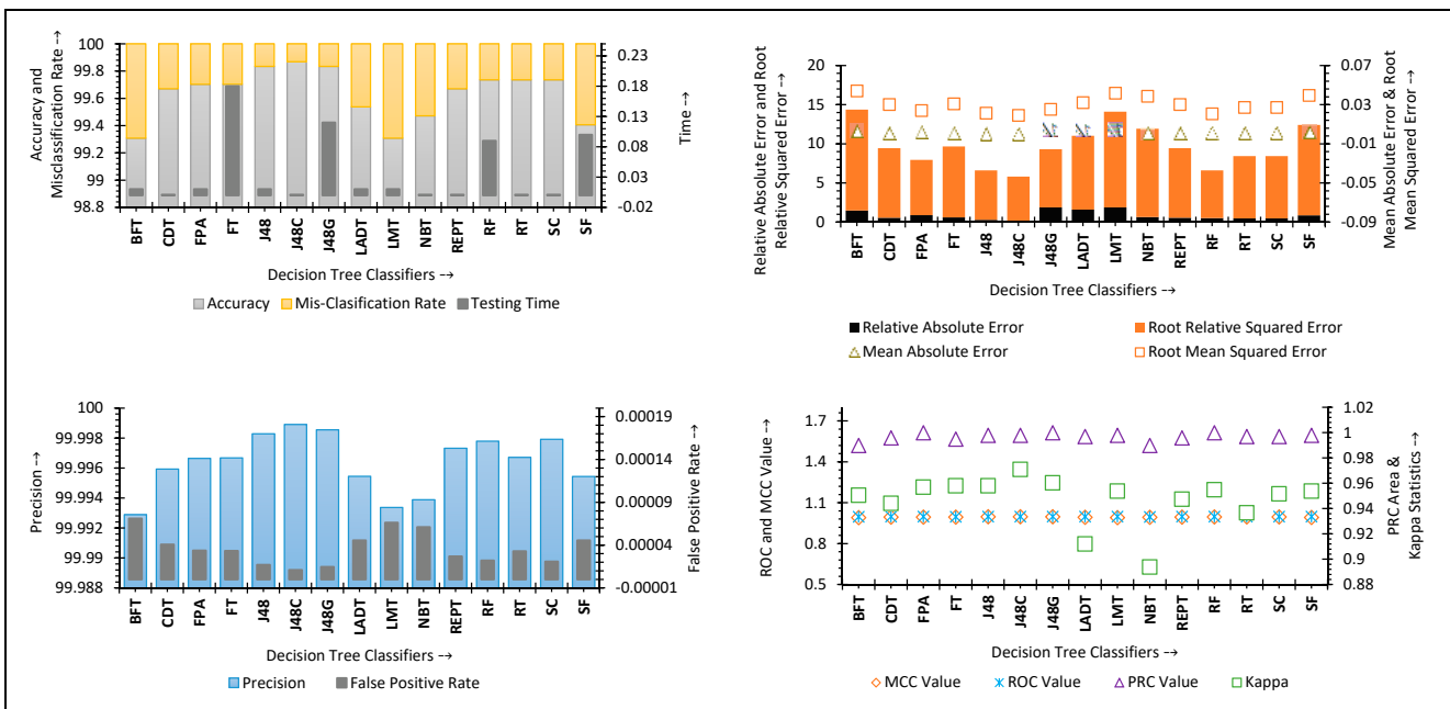
Figure 7. Performance of decision tree classifiers for CICIDS2017 dataset.
