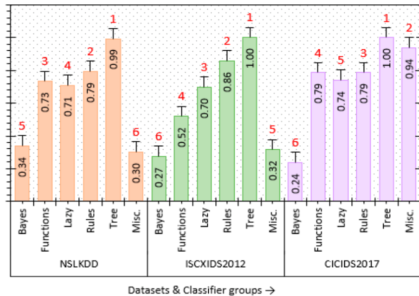
Figure 4. Weights and ranks of supervised classifier groups.
