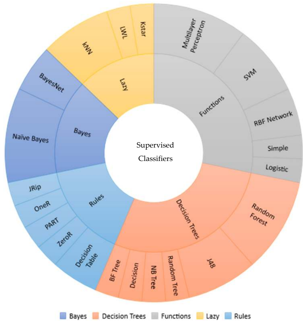
Figure 1. Usage statistics of supervised classifiers.
