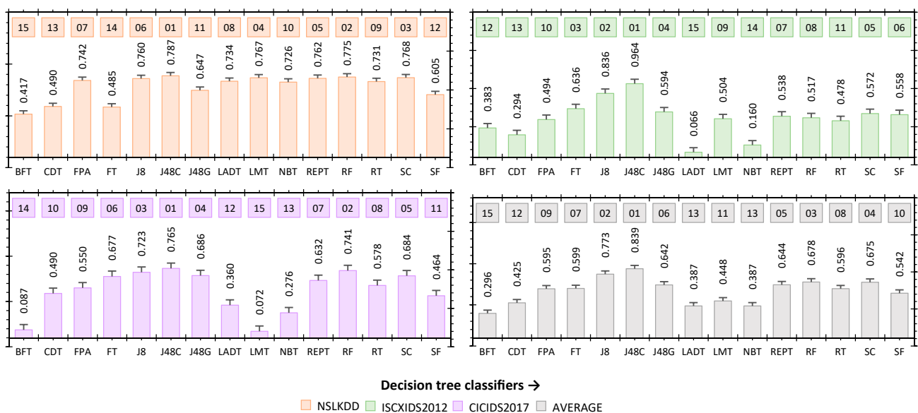
Figure 8. Techniques for Order Preference by Similarity to the Ideal Solution (TOPSIS) weights and ranks of decision tree classifiers for NSLKDD, ISCXIDS2012 and CICIDS2017 dataset.
