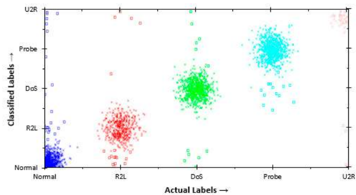
Figure 12. Classification of J48Consolidated on NSL-KDD dataset.
