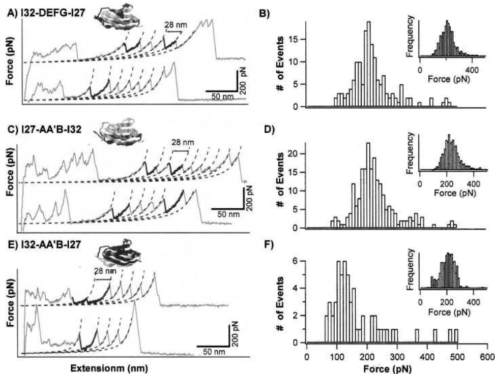
Figure 5. Hybrid Ig domains I32-DEFG-I27, I27-AA'B-I32, and I32-AA'B-I27 exhibit duality in their mechanical stability. (A,C, and E) Typical force–extension curves of (GB1-I32-DEFG-I27) 4 , (GB1-I27-AA'B-I32) 4 , and (GB1-I32-AA'B-I27) 4 , respectively. The unfolding events of GB1 are colored in gray. The unfolding events with \Delta Lc of \sim 28 nm correspond to the unfolding of hybrid Ig domains and are in black. It is of note that the number of GB1 unfolding events in the force–extension curves are much greater than the number of the unfolding events of hybrid Ig domains. (B,D, and F) Unfolding force histograms of I32-DEFG, I27-AA'B-I32, and I32-AA'B-I27 domains in the heteropolyproteins. The number of events in these histograms is 154, 211, and 57, respectively. Insets in B, D, and F are unfolding force histograms of GB1 domains in the heteropolyproteins, respectively. The number of events is 570, 1199, and 377, respectively.
