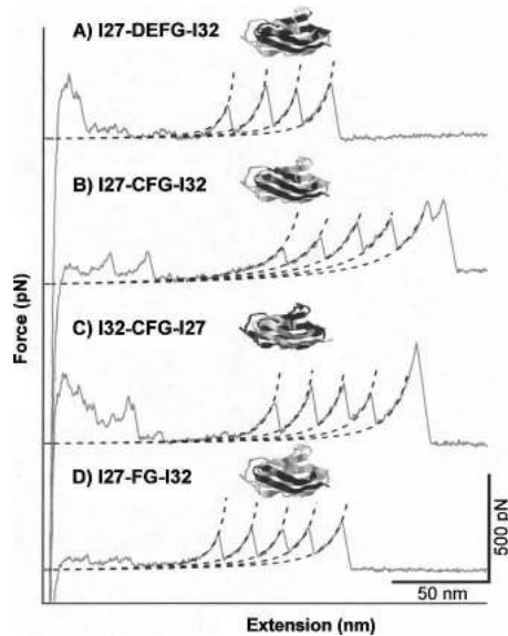
Figure 4. Typical force–extension curves of heteropolyprotein (A–D) (GB1-I27-DEFG-I32) 4 , (GB1- I27-CFG-I32) 4 , (GB1- I32-CFG-I27) 4 , and (GB1-I27-FG-I32) 4 . The force–extension curves of these heteropolyproteins are characterized by long featureless spacers followed by the unfolding events of GB1 domains, which corresponds to the stretching of hybrid Ig domains that unfold at low force (below our detection limit). Dotted lines are WLC fits to the experimental data.
