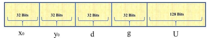
FIGURE 5. The key structure of CTC-IES
