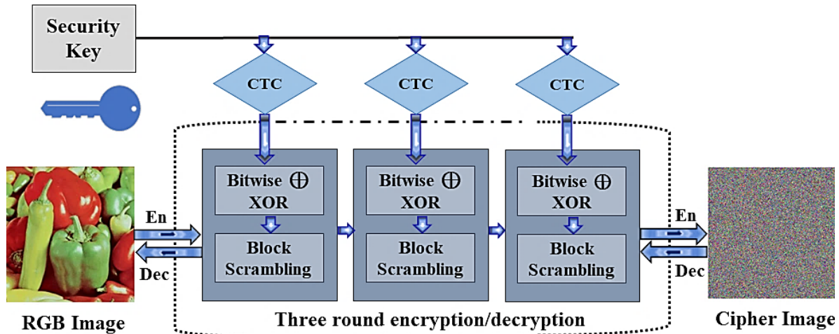
FIGURE 4. Keyframes encryption process
