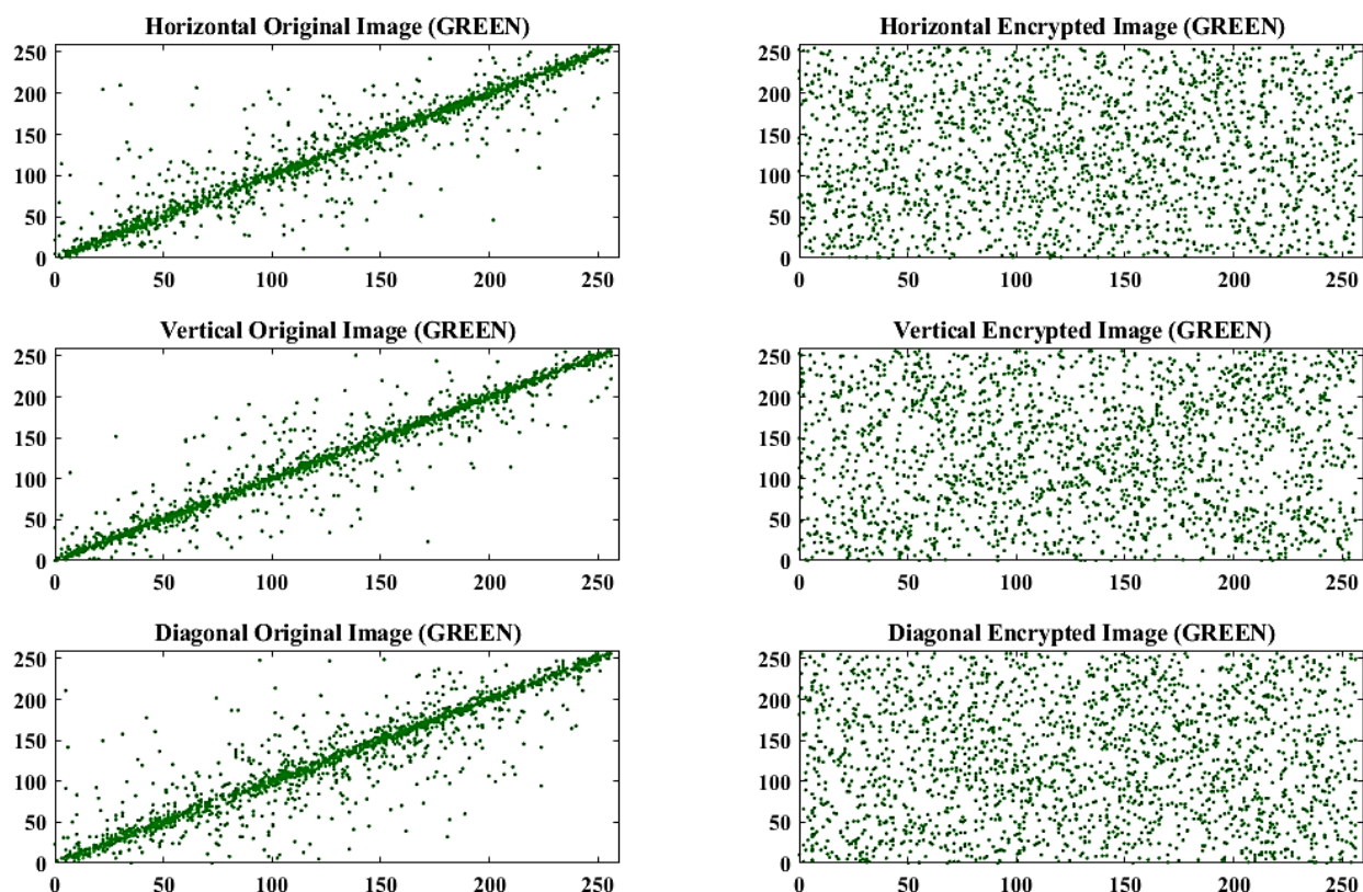
FIGURE 11 Distribution of two neighboring pixels (horizontally, vertically, and diagonally) in the plain keyframe and encrypted keyframe image (green component).
