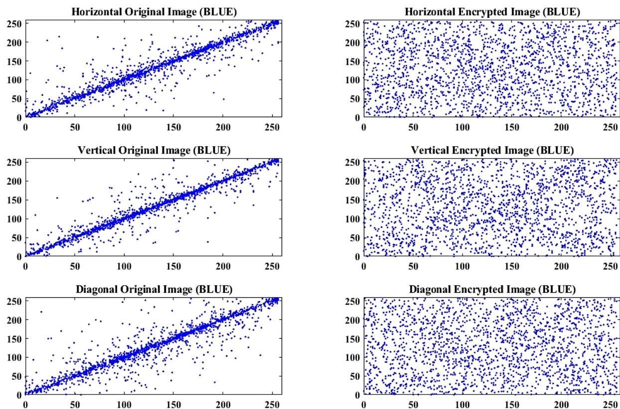
FIGURE 12 Distribution of two neighboring pixels (horizontally, vertically, and diagonally) in the plain keyframe and encrypted keyframe image (blue component).
