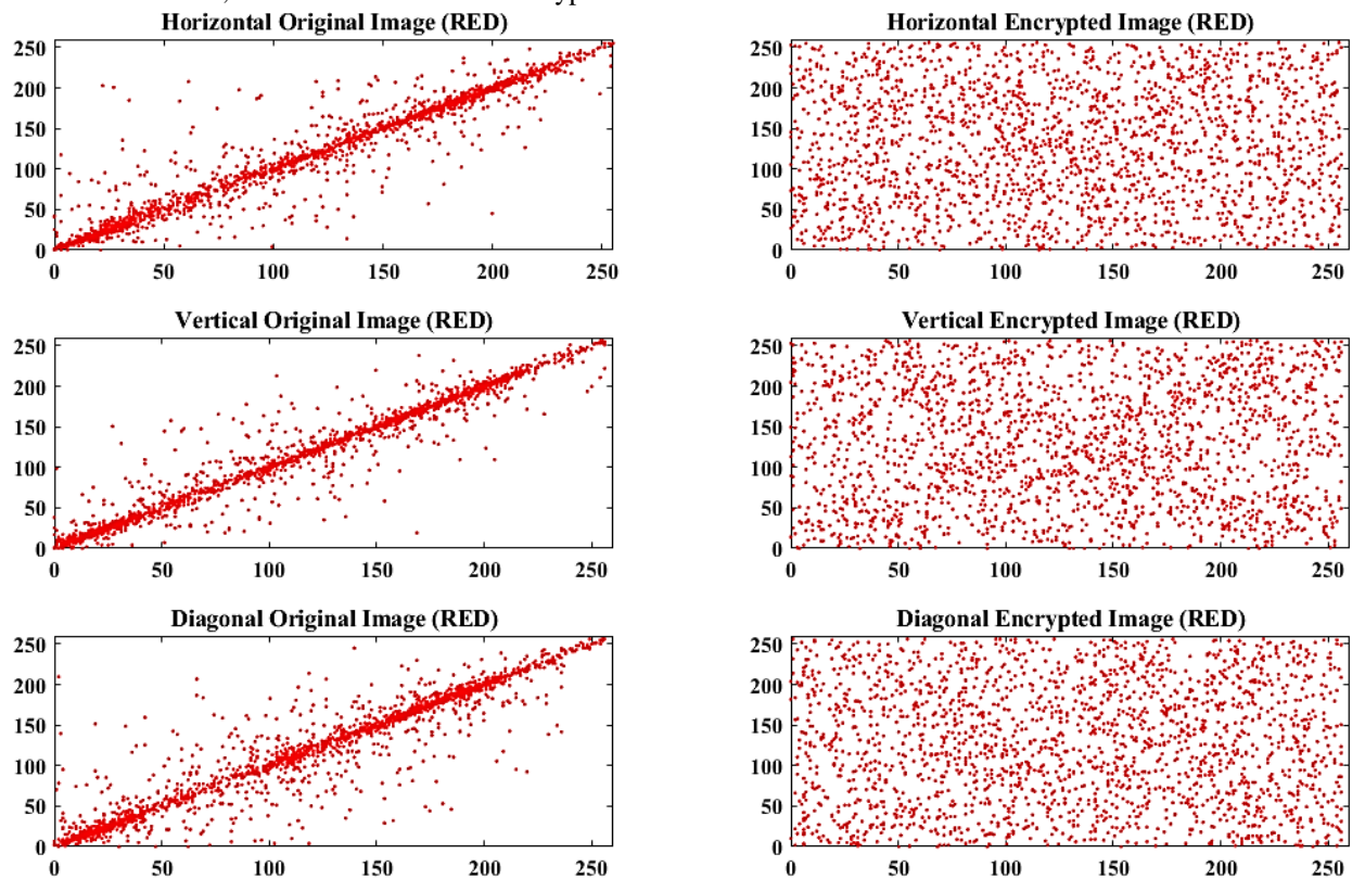
FIGURE 10 Distribution of two neighboring pixels (horizontally, vertically, and diagonally) in the plain keyframe and encrypted keyframe image (red component).
