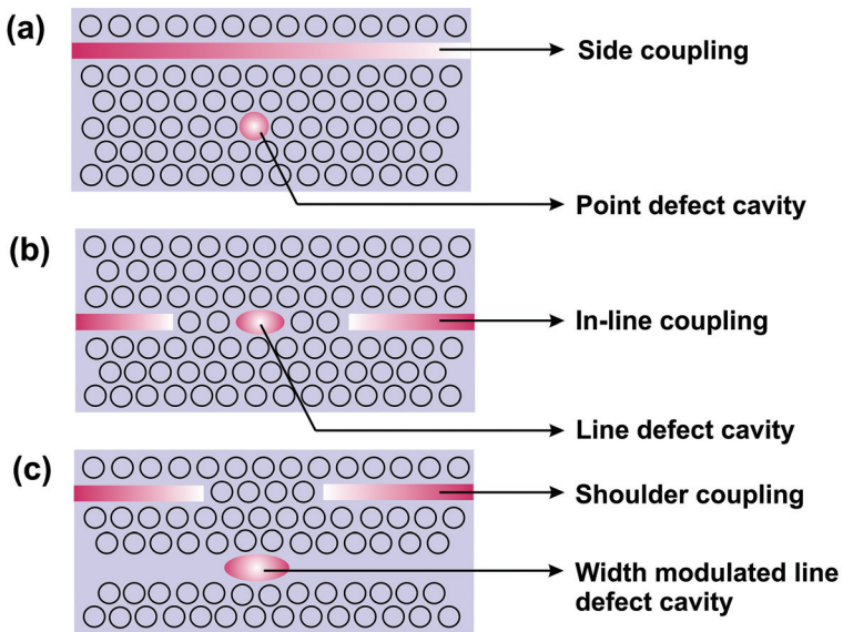
Figure 4. Schematic representation of nanocavities along with various coupling schemes: (a) a point-defect nanocavity with side coupling with the waveguide, (b) a line-defect nanocavity with in-line coupling with the waveguide, and (c) a width-modulated line defect nanocavity with shoulder coupling with the waveguide.
