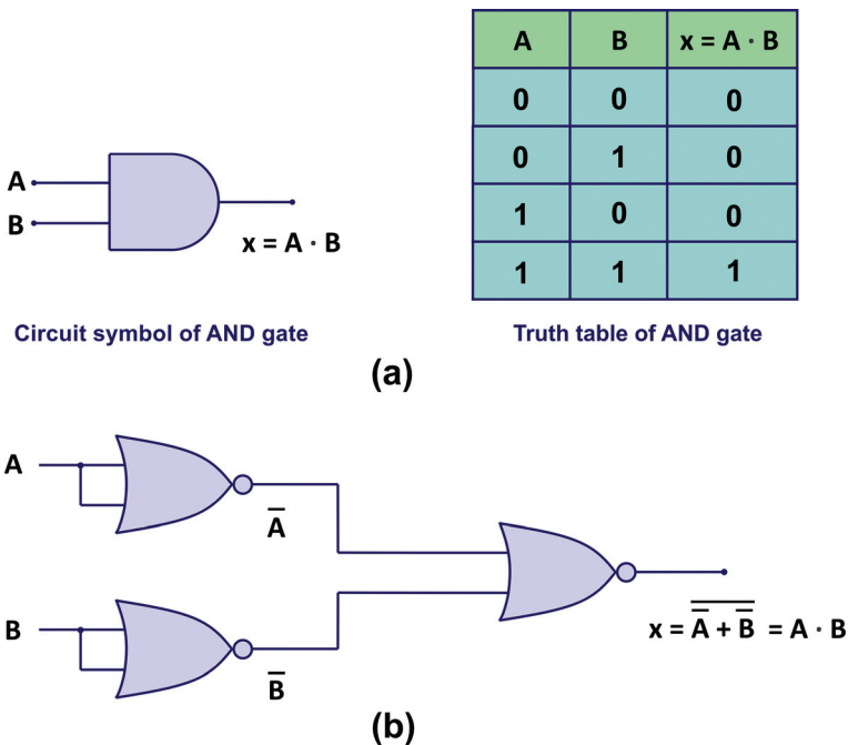
Figure 8. (a) Circuit symbol and truth table of AND gate and (b) implementation of AND operation using NOR gates.
