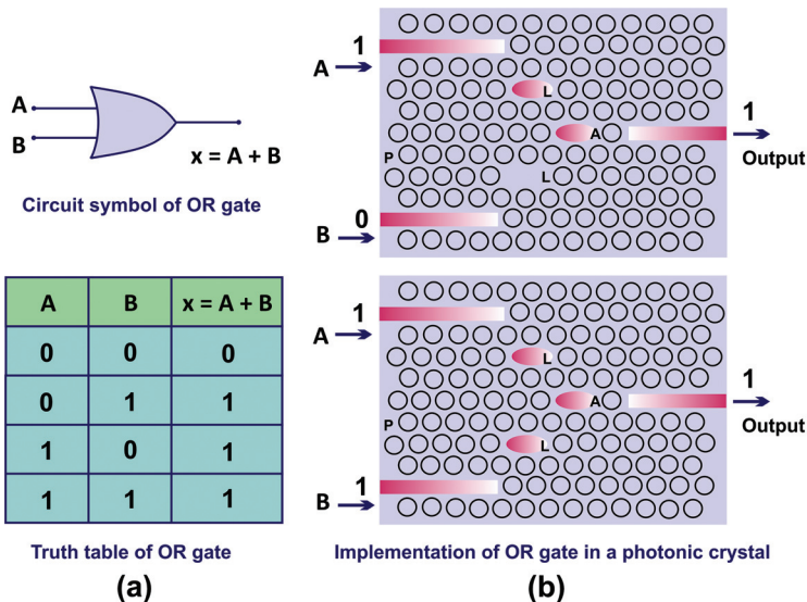
Figure 7. (a) Circuit symbol and truth table of OR gate and (b) implementation of OR gate operation in a photonic crystal slab.
