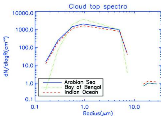
Fig. 2. Spectra at the cloud top for sulphate and salt based droplets for the three regions.
