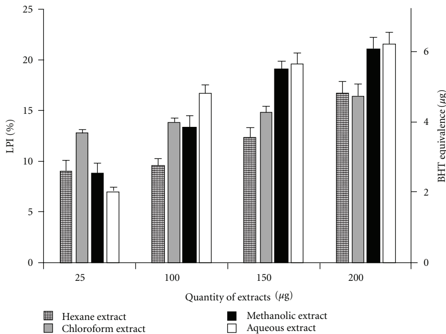
FIGURE 3: Inhibitory effect of C. cinereum extracts on lipid peroxidation. Percentage LPI values are given as mean \pm SD ( n = 3, P < .05 ). BHT equivalence (in \mu\text{g} ) is shown for all extract concentrations.
