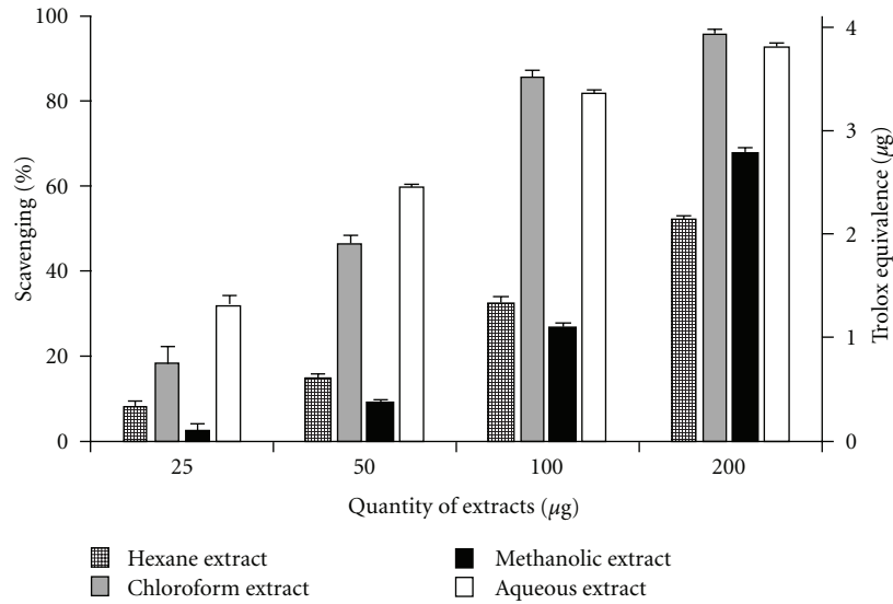
FIGURE 2: ABTS •+ radical scavenging activity of C. cinereum extracts in different concentrations with Trolox equivalence (in \mu\text{g} ). Data expressed as mean \pm SD ( n = 3, P < .05 ).
